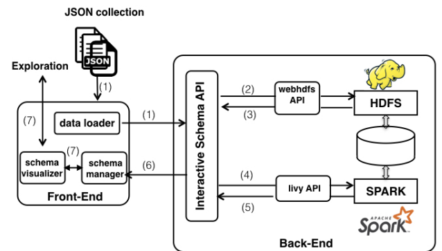
Figure 4: System architecture.
