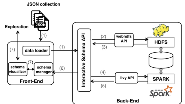
Figure 4: System architecture.
