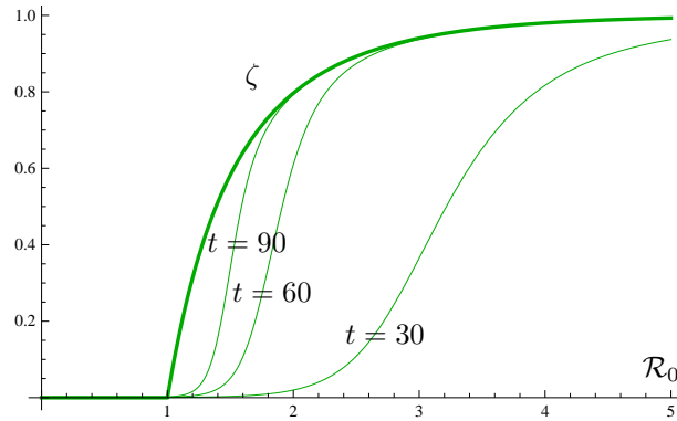
FIGURE 2. The epidemic size \zeta as a function of the basic reproduction ratio \mathcal{R}_0 in the simplest SEIR model corresponding to (6)-(9) exhibits a clear phase transition at \mathcal{R}_0 = 1 (thick curve). The other curves represent r(t) taken for t = 30, 60, 90 , for which equilibrium is not yet achieved. In practice, varying \mathcal{R}_0 is achieved by acting on the q factor in (25)-(28).
