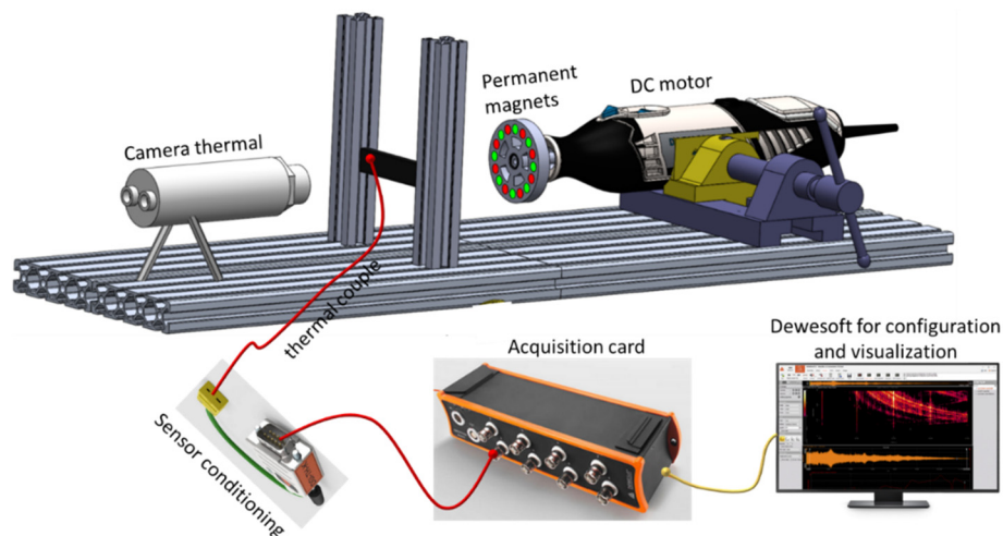
Figure 3. Experimental setup of the induction heating (IH) equipment.
