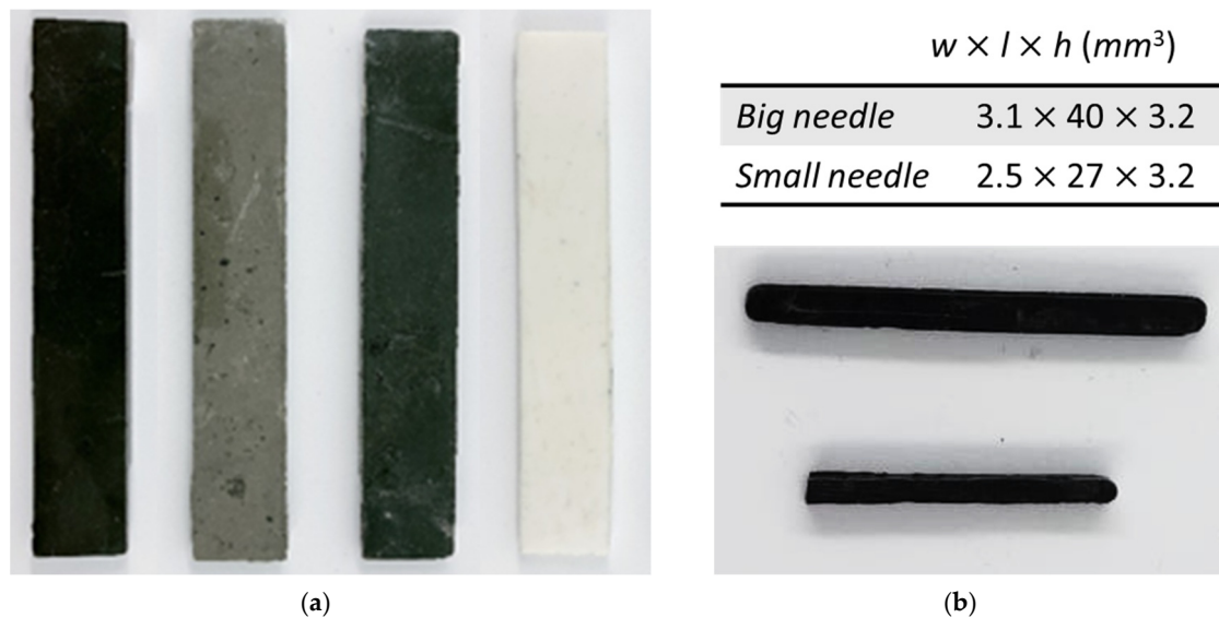
Figure 2. (a) Rectangular samples (from left to right): Three ferromagnetic composites filled with iron oxide, nickel, or manganese; pure ABS is also included. (b) Samples of needle shape.
