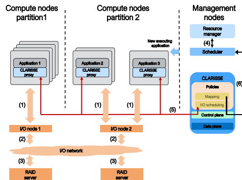
Figure 2: Framework overview.
