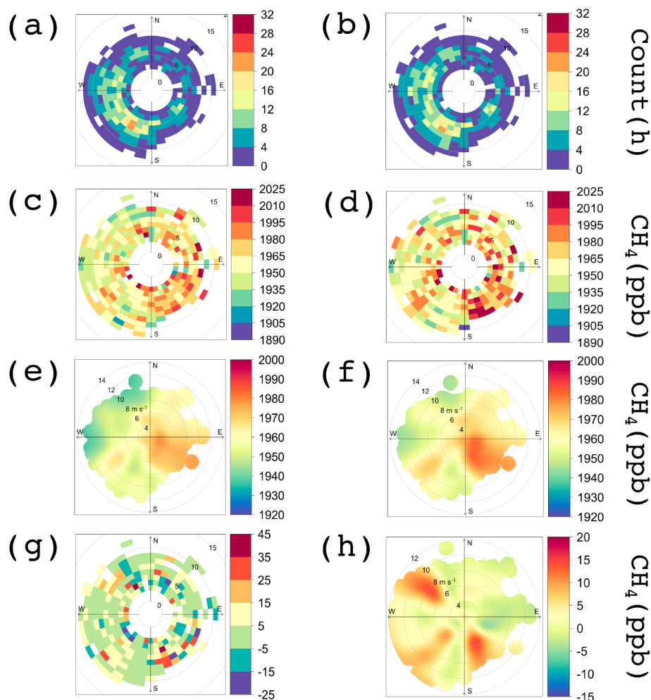
Figure 4. Frequency and bivariate polar plots of \text{CH}_4 background for Indianapolis using data from 12:00–16:00 LST, November 2014 through December 2016 given two different criteria (Table 1). (a) Polar histogram indicating a number of hourly measurements available using criterion 1. (b) Same as (a) only for criterion 2. Differences between (a) and (b) are due to slight differences in data availability at the considered towers. (c) Polar frequency plot of the \text{CH}_4 background using criterion 1. (d) Same as (c) only for criterion 2. (e) Polar bivariate plot of \text{CH}_4 background using criterion 1. (f) Same as (e) only for criterion 2. (g) Polar frequency plot of difference between the backgrounds: criterion 2 – criterion 1. (h) Same as (g) but shown with a bivariate polar plot.
