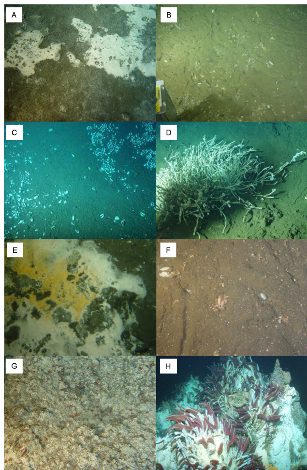
Figure 2. Images of studied assemblages at seeps: (a) S_Mat and S_Gast, (b) S_VesA, (c) S_VesP, (d) S_Sib and S_Sib_P and vents: (e) V_Mat, (f) V_VesA, (g) V_Alv and (h) V_Sib.
