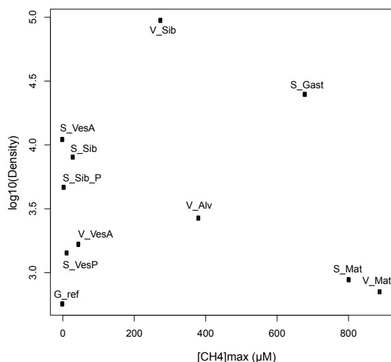
Figure 4. Log-transformed macrofaunal densities according to maximum methane concentrations in assemblages.
