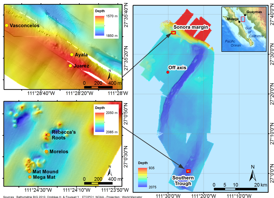
Figure 1. Localisation of the study sites on the Sonora margin cold seeps (Ayala, Vasconcelos and Juarez sites), the Southern Trough hydrothermal vents (Rebecca's Roots, Mat Mound, Morelos and Mega Mat sites) and the Guaymas Basin off-axis reference site.
