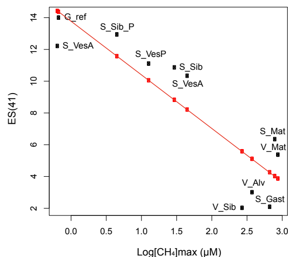
Figure 6. Logarithmic regression between species richness, ES(41) , and maximum methane concentration in all macrofaunal assemblages. Black squares represent observed data points and red squares represent fitted values.
