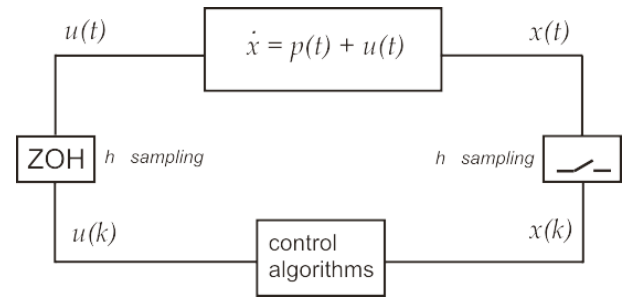
Fig. 1. Controlled system by discrete control algorithms.
