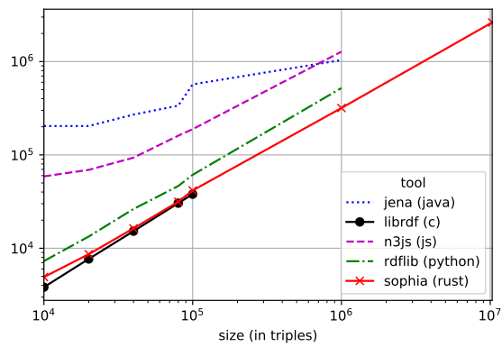
Figure 2: Memory (in kB) used to load an NT file in memory
