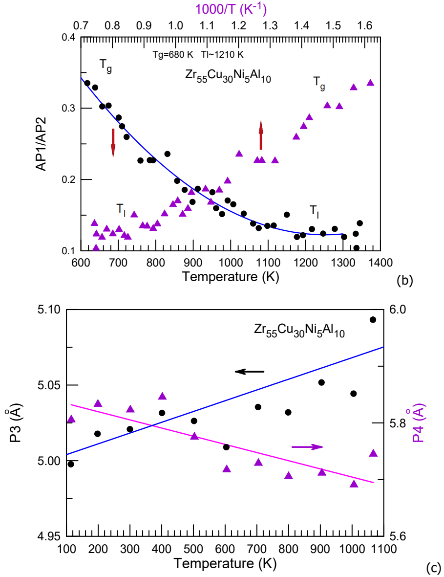
Fig. 3. Positions of P1 and P2 in the first coordination shell (a) and the ratio of the corresponding peak areas ( AP1/AP2 ) (b) as a function of temperature (a,b) and inverse temperature in (b). The positions of P3 and P4 as a function of temperature (c). The arrows in (a and c) indicate Y-axes corresponding to the data while the arrows in (b) indicate the corresponding X-axes. The insert in (a) is schematic representation of atomic redistribution within and between the first and higher order coordination shells leading to continuous structure changes in metallic liquids on heating and cooling leading to redistribution of the atomic number density as indicated by the red double side arrow.
