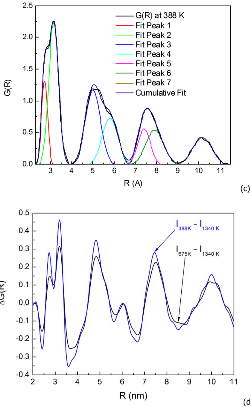
Fig. 2. Fitting of four G(R) maxima (black curve) from 0.23 to 1.15 nm using seven Gaussian functions related to P1 – P7 (as indicated). The curves in (a) correspond to 1340 K, curves in (b) to 675 K while the curves in (c) to 388 K. The baseline was subtracted prior to fitting according to the minima at about 2.2, 4, 6.7, 9 and 11.5 Å. The inset in (b) shows R_{50}^i value at
