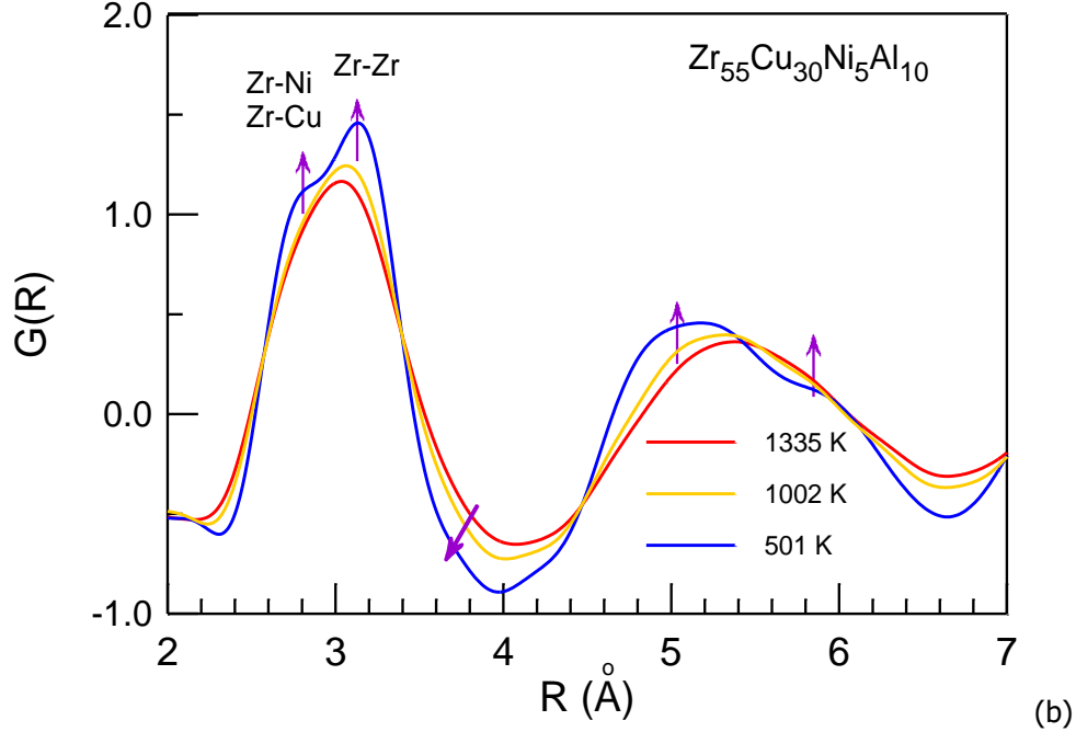
Fig. 1. (a) The experimental structure factor S(Q) at 1335 and 388 K calculated from the corresponding XRD intensity profile after the necessary corrections. (b) three typical G(R) functions. Violet arrows (upward) show intensification of two sub-peaks responsible for Zr-(Cu,Ni) and Zr-Zr atomic interactions in the first coordination shell and two sub-peaks at 0.5 and 0.58 nm in the second coordination shell. The arrow focusing downward-left indicates a decrease in the number of high R value atomic interactions on cooling.
