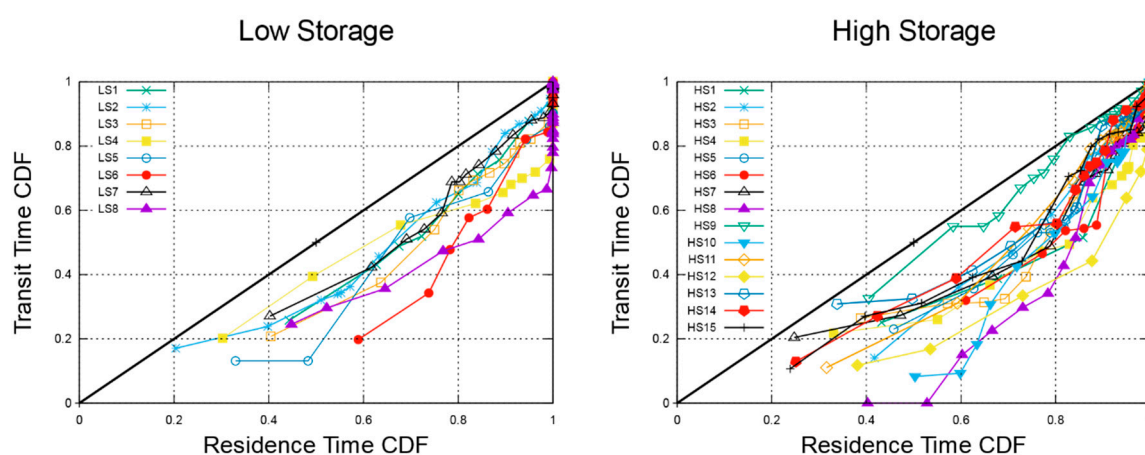
Figure 12. StorAge Selection (SAS) functions for low-storage (LS) and high-storage (HS) conditions. SAS functions are represented in a cumulative (CFD, cumulative density function) form by plotting for various times the cumulative transit-time probability versus the cumulative residence-time probability.
