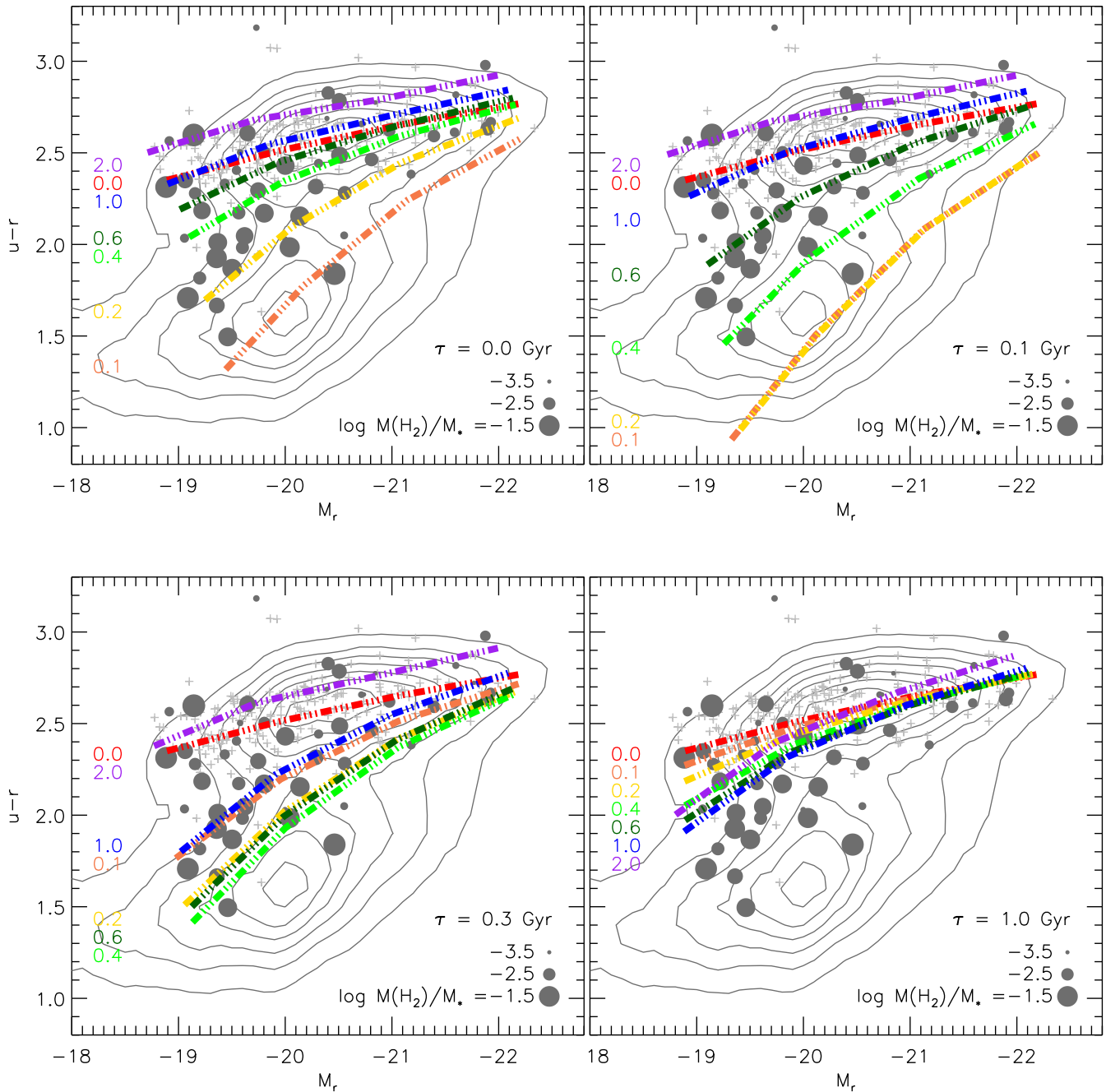
Figure A1. Model isochrones for a simple scenario in which cold gas drops onto a red sequence galaxy and initiates some star formation activity. The total mass of stars formed is 3 \times 10^8 M_{\odot} . Panels show four different star formation histories for the late burst, including a delta function ( \tau = 0 Gyr) and delayed tau models with \tau = 100 Myr, 300 Myr, and 1 Gyr. Dashed lines indicate the location of the “red sequence” at the times indicated (in Gyr, relative to the beginning of the burst). Contours and other symbols are the same as in Figure 7, with the exception that here the symbol size is the normalized H_2 mass. In the \tau = 0 panel, an isochrone earlier than 0.1 Gyr would show yet bluer colours; in the other panels, the minimum in u - r colours can be seen where the isochrones change from becoming bluer with time to becoming redder.
