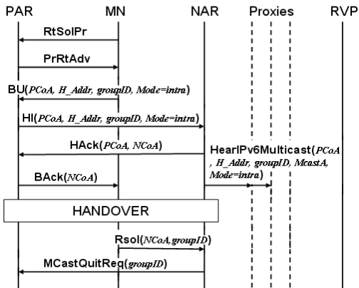
Figure 3. Intra-RVP-domain handover procedure.
