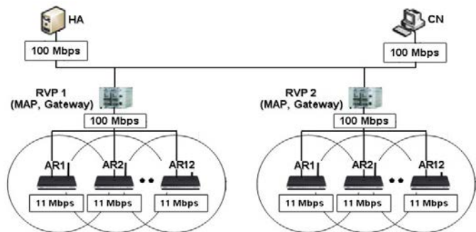
Figure 5. Simulation’s network topology.
