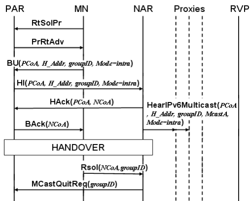
Figure 3. Intra-RVP-domain handover procedure.
