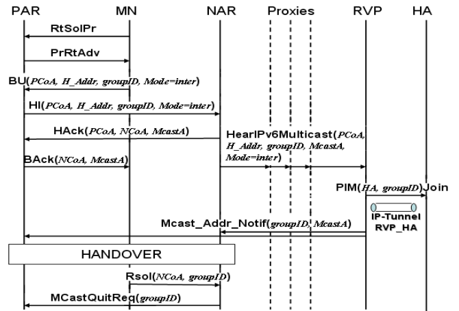
Figure 2. Inter-RVP-domain handover procedure.
