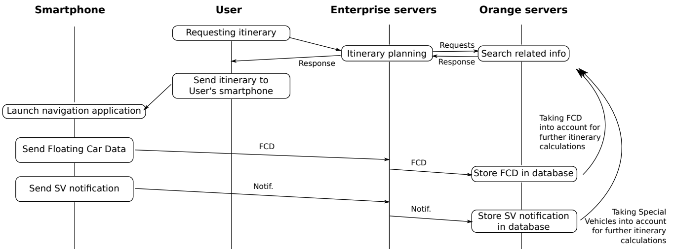
Figure 2. Sequence diagram
