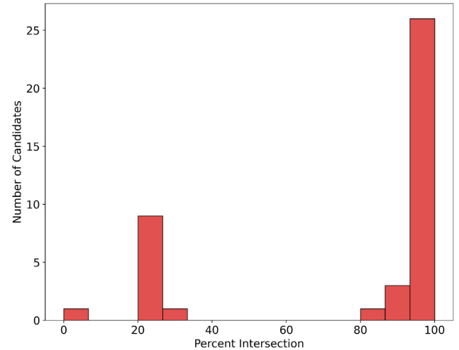
Figure 5. Overlap ratio between the initial and the most up-to-date 90 per cent credible regions of all GW candidate events during O3 (given that both sky localizations were available). Note that the overlapping regions can be discontinuous.
