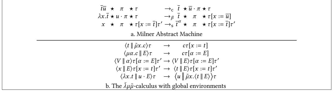
Figure 11. Milner Abstract Machine and \bar{\lambda}\mu\tilde{\mu} -calculus
