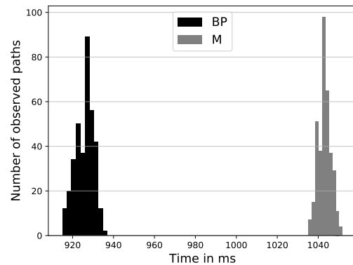
Fig. 4. Histogram showing the observed times elapsed between the rising edge and falling edge of the photoelectric sensor next to the first sorting pusher (BP in black and M in grey) in the observed timed paths.
