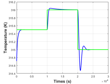
Fig. 2. Output (blue) and reference (green) temperatures
