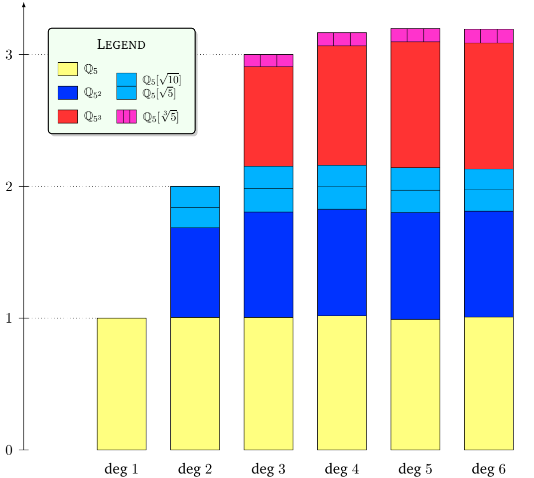
Figure 2: Average number of roots of a polynomial in various extensions. Sample of 500,000 polynomials over \mathbb{Z}_5 picked uniformly at random.
