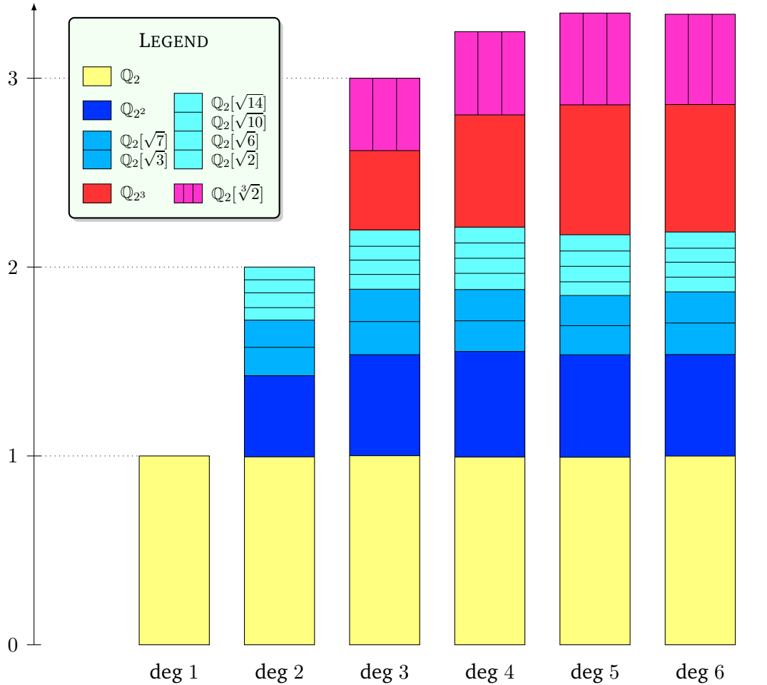
Figure 1: Average number of roots of a polynomial in various extensions. Sample of 500,000 polynomials over \mathbb{Z}_2 picked uniformly at random.
