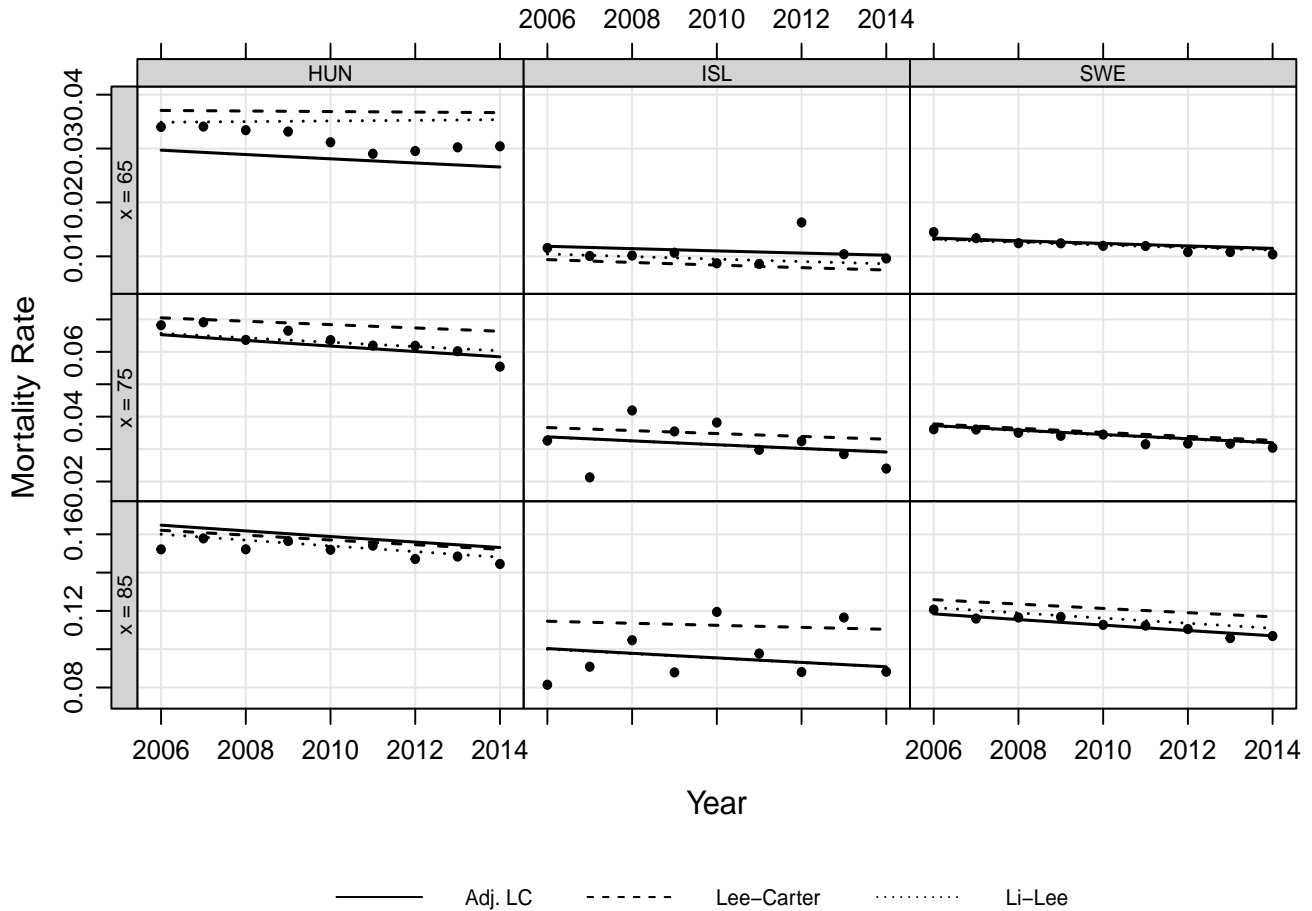
Figure 3: Mortality rates over the period 2006-2014: Observed mortality (black circles), credibility adjusted forecast (solid line), Lee and Carter's forecast (dashed line) and the Li and Lee (dotted line), for ages 65, 75 and 85.
