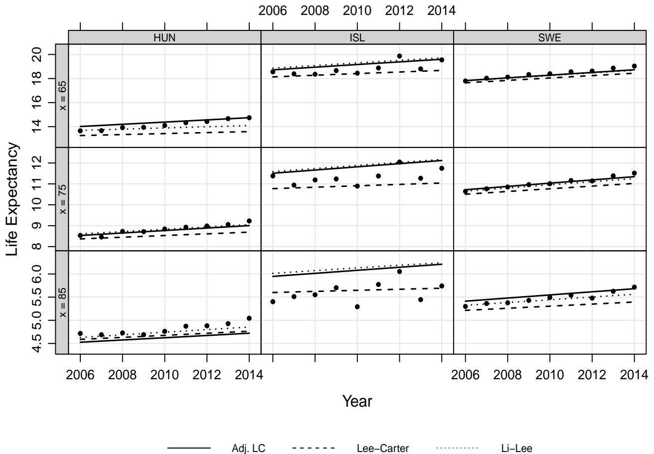
Figure 4: Life expectancy over the period 2006-2014: Observed life expectancy (black circles), credibility adjusted forecast (solid line), Lee and Carter’s forecast (dashed line) and the Li and Lee (dotted line), for ages 65, 75 and 85.
