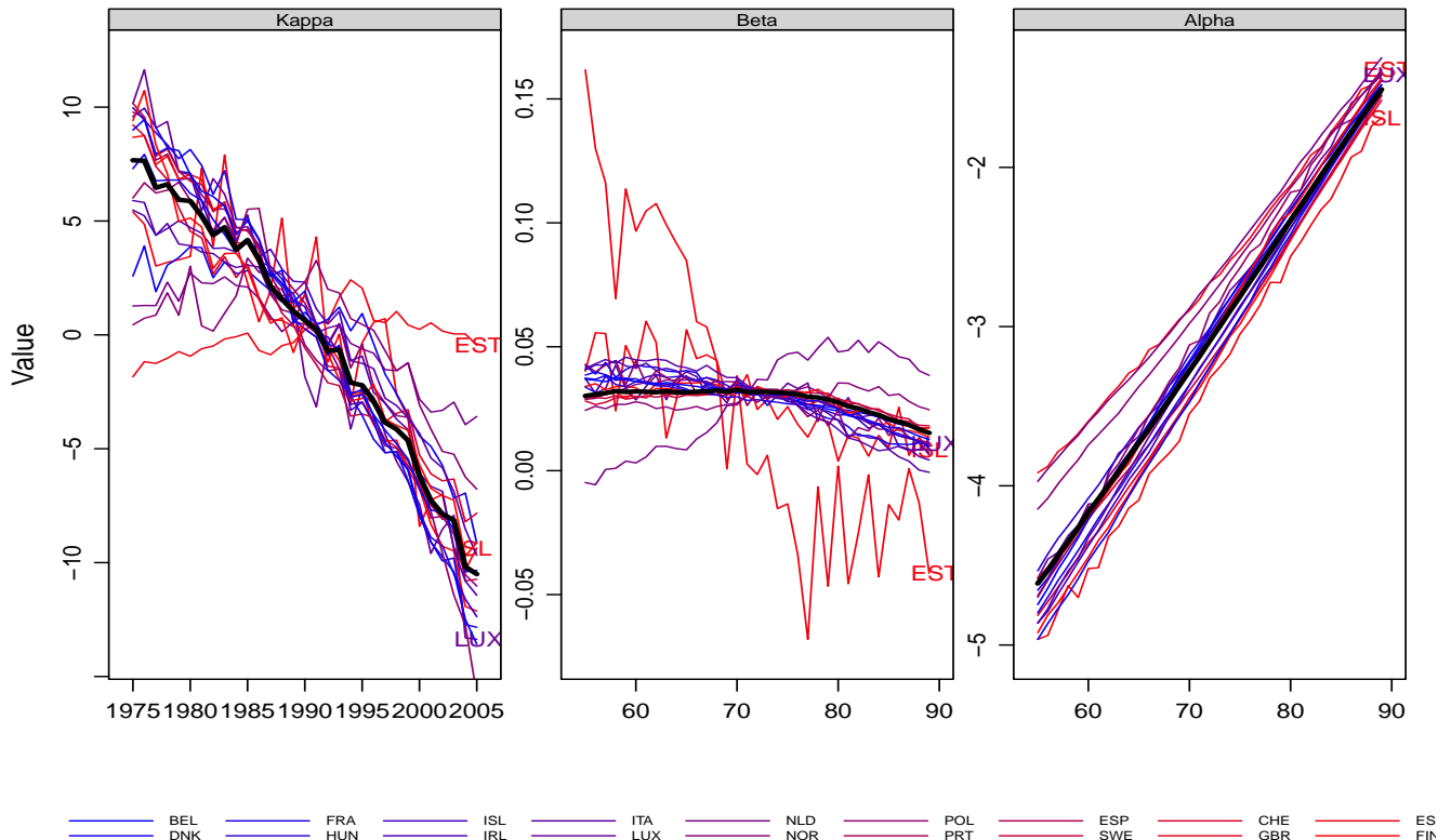
Figure 1: The estimated parameters \alpha_x^i, \beta_x^i and \kappa_t^i for the 18 countries as well as the aggregate parameters \alpha_x^\bullet, \beta_x^\bullet and \kappa_t^\bullet in black.
