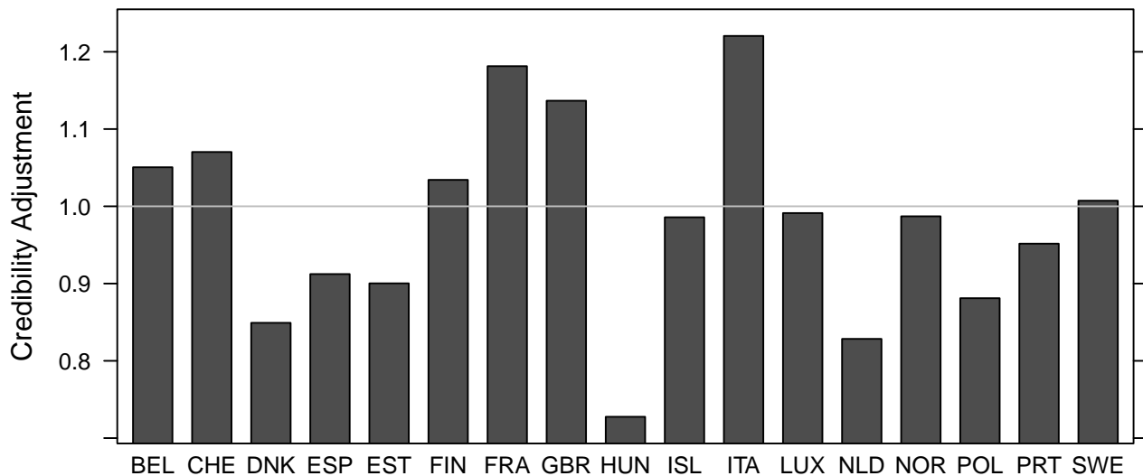
Figure 2: Next-period adjustment of the joint- \kappa model based on the credibility adjustment in Equation (3.8)
