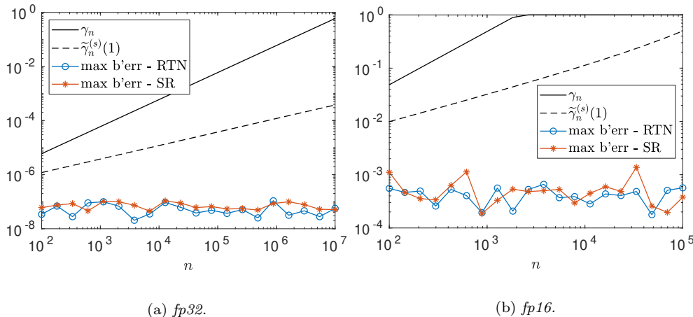
Fig. 5.3: Computed backward errors of inner products for data sampled uniformly from [-1, 1] in fp32 (a) and fp16 (b). For each value of n we perform the computation 10 times and plot the maximum backward error for each rounding mode.
