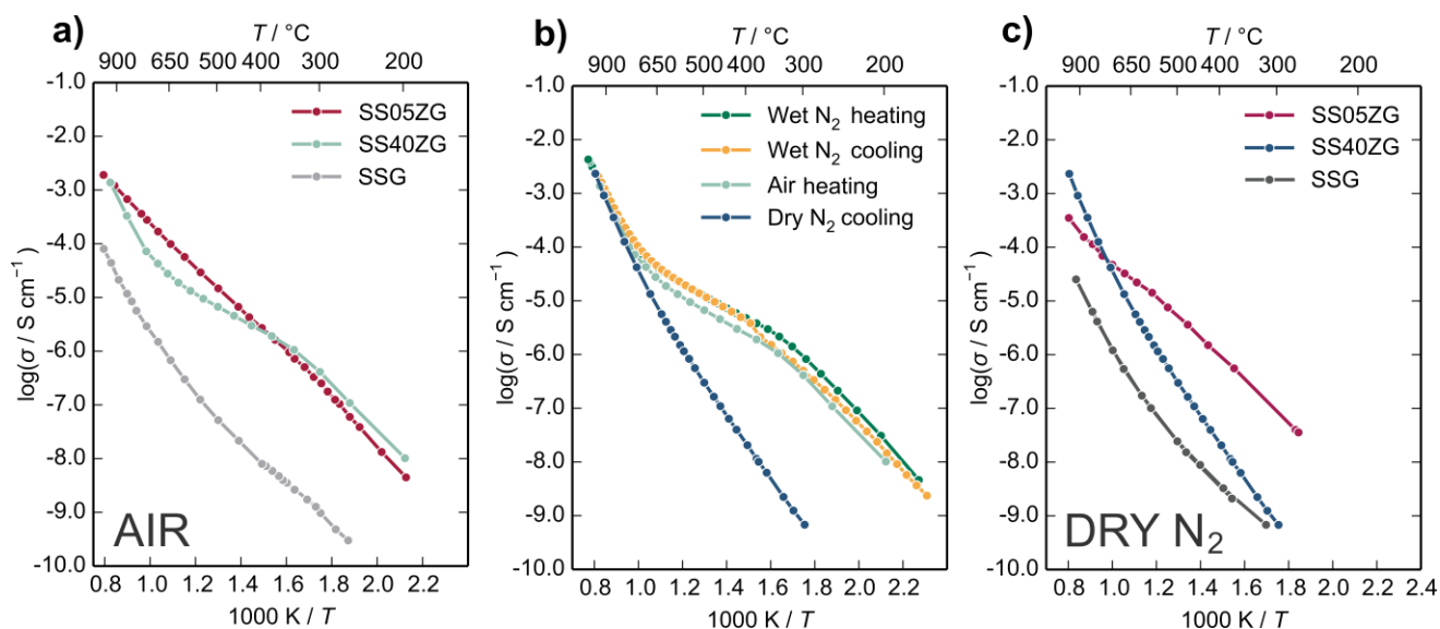
Figure 2. Conductivity as a function of temperature for SSZ40GO and related compounds. a) comparison of conductivities in air for the different compounds. b) conductivity under different atmospheres for SSZ40GO c) comparison between conductivities in dry nitrogen for the different compounds. Data shown for SSGO and SSZ05G are from both heating and cooling cycles.
