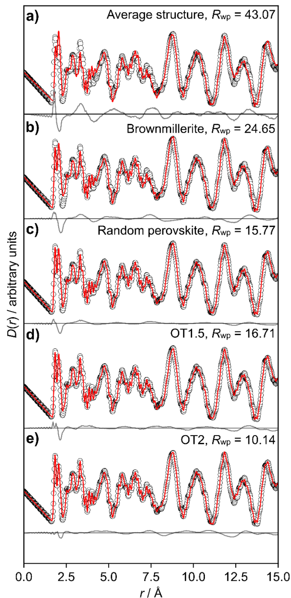
Figure 6. Fit of various local structure models (red curve) to the measured PDF (black markers) data of SSZ40GO. Difference curves are shown in grey. The R_{wp} values given are calculated for 1.5 \text{ \AA} \leq r \leq 8 \text{ \AA} to reflect the fit to the local structure.
