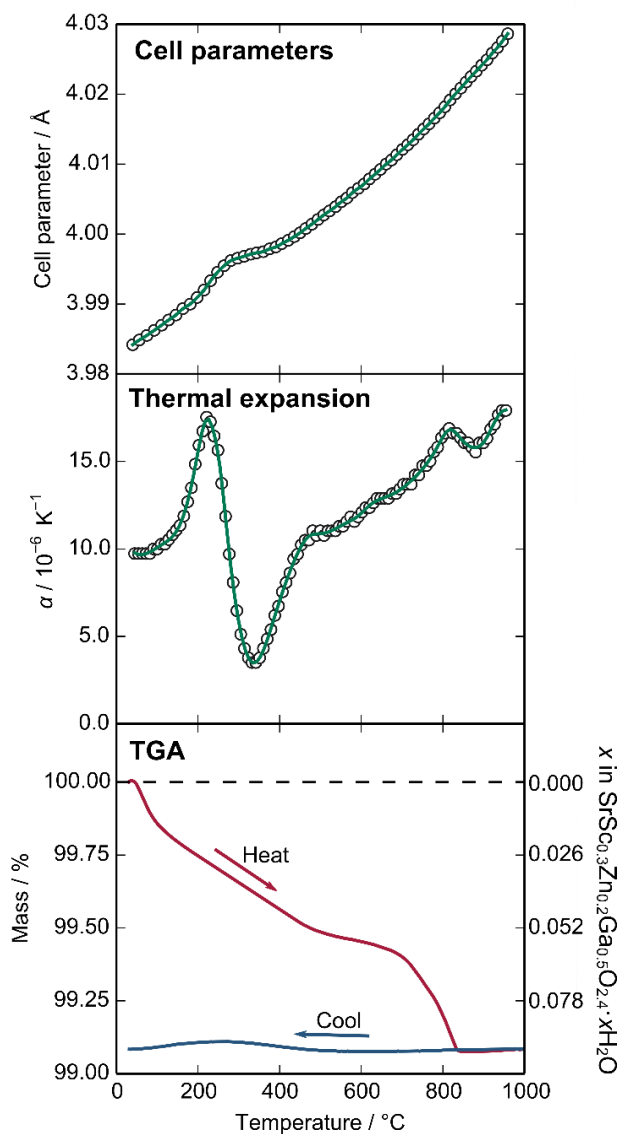
Figure 3. SSZ40GO cell parameter evolution with temperature from variable temperature X-ray diffraction (top panel) and derived thermal expansion ( d\alpha/dT ) (middle). Thermogravimetric analysis over the same temperature range (bottom) on both heating and cooling cycles. Cell parameters on cooling are shown in the SI.
