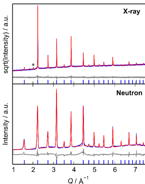
Figure 1. Rietveld fits of a simple Pm\text{-}3m perovskite model against the room temperature X-ray (top) and neutron (bottom) data for SSZ40GO. Blue, red and grey curves show the observed, calculated and difference curves respectively. Blue tick marks indicate the expected peak positions. The peak highlighted with an asterisk is as a result of W\text{ L}\alpha incident X-ray contamination. X-ray data are shown on a square root scale to emphasize weaker features.
