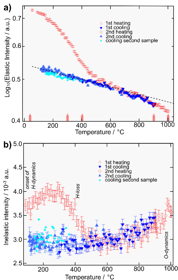
Figure 5. a) Elastic intensity as a function of temperature summed over all Q -values (0.2–1.75 \text{\AA}^{-1} ). Multiple heating and cooling cycles are shown. The dashed line is a guide to the eye showing the expected decrease in intensity due to Debye-Waller effects. Temperatures where QENS spectra were subsequently measured are indicated by the red markers on the temperature axis. b) Inelastic intensity at 2 \mu\text{eV} energy transfer as a function of temperature summed over all Q -values (0.2–1.75 \text{\AA}^{-1} ). Key features are labelled with the dynamic processes to which they have been attributed.
