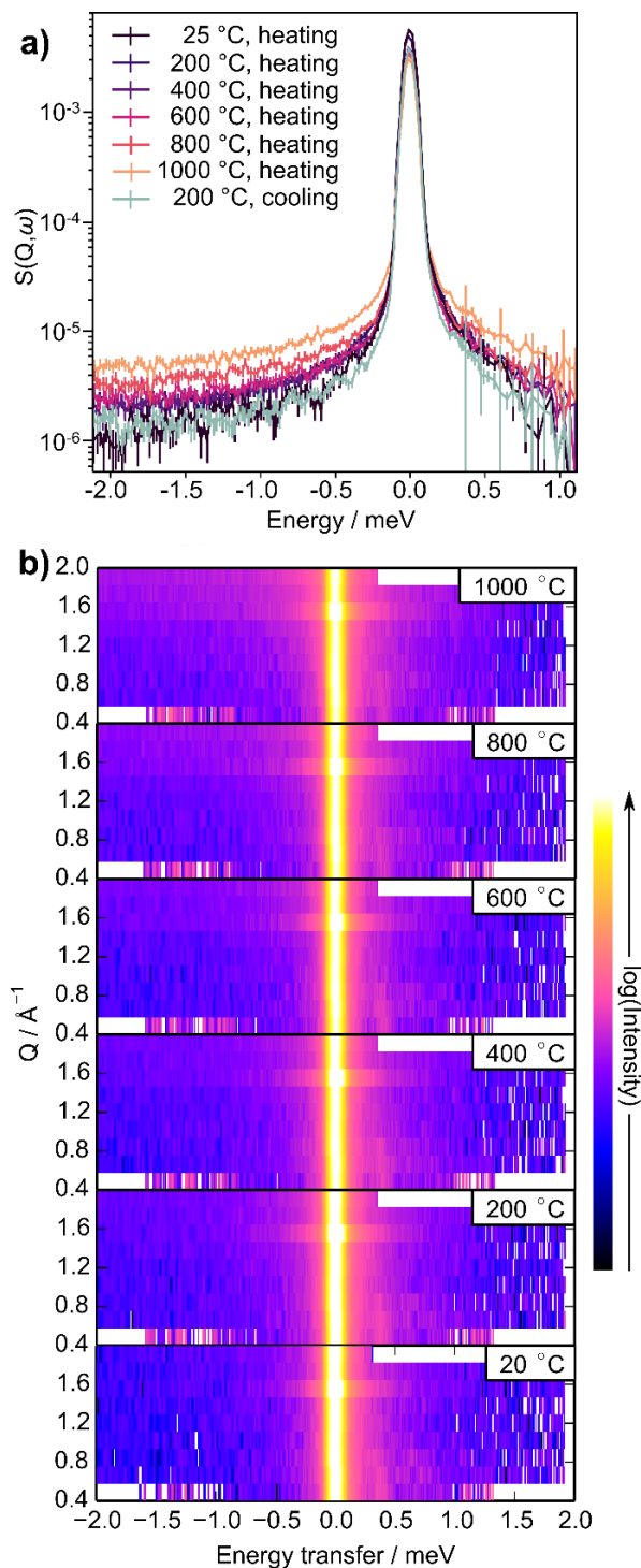
Figure 4. a) Plot of the scattering function S(\omega) at Q = 1.92 \text{ \AA}^{-1} showing the QENS broadening of the elastic peak. b) Colour maps of S(Q, \omega) at different temperatures to show the evolution of the QENS broadening at high temperatures and that this is enhanced at high Q .
