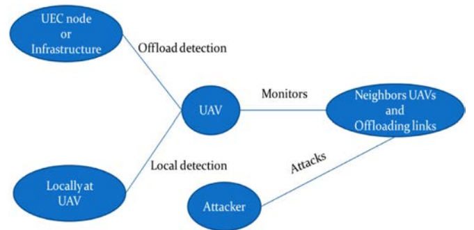
Fig. 2. Illustration of attack detection process in UEC network.
