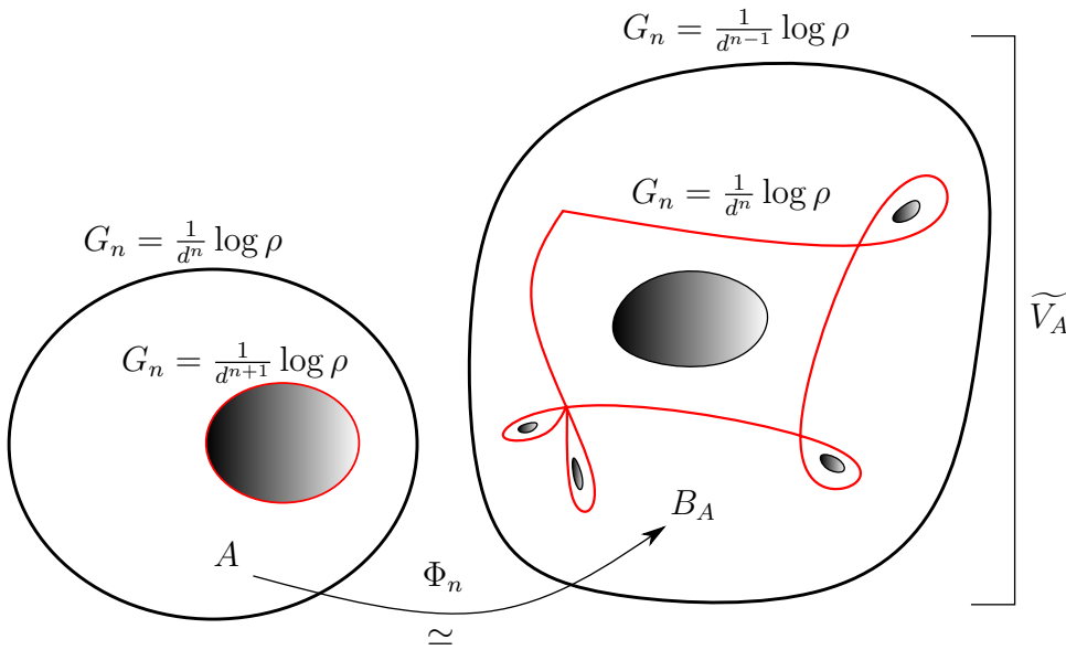
FIGURE 8. The patching procedure when A \neq A_\star
