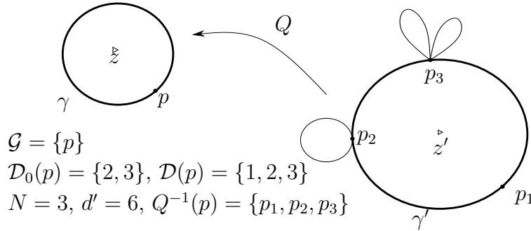
FIGURE 5. Example where \mathcal{Q}(p) \subset \gamma' but \mathcal{D}_0(p) \subsetneq \mathcal{D}(p)
