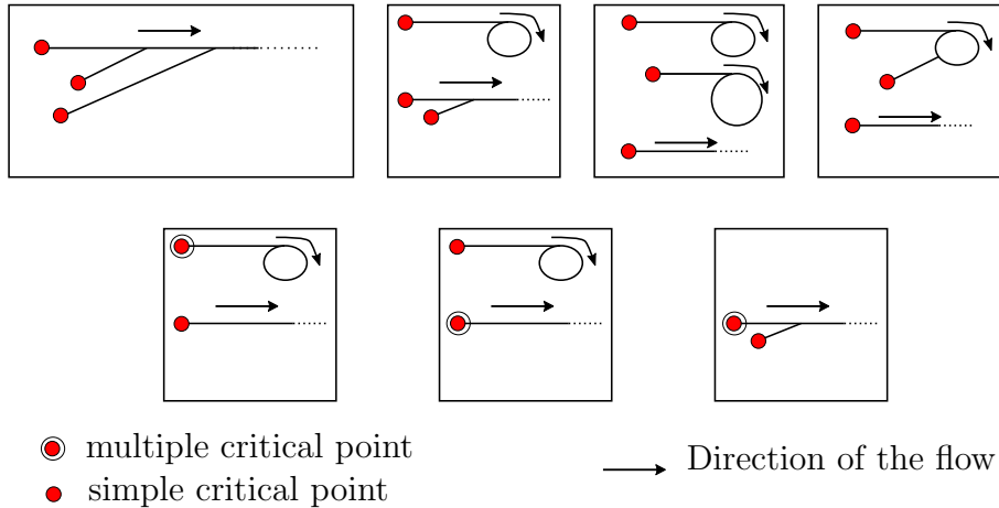
FIGURE 12. Asymmetrical special critically marked dynamical graphs of degree 4
