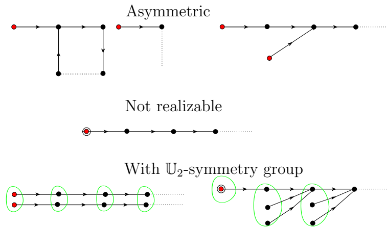
FIGURE 4. Special critically marked dynamical graphs of degree 3. Circled red dots are multiple critical critical points
