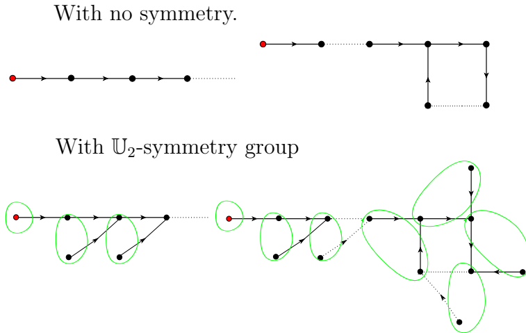
FIGURE 3. Special critically marked dynamical graphs of degree 2: the critical point is marked in red, and \mathbb{U}_2 -orbits in green
