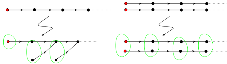
FIGURE 2. Two examples of non-asymmetric graphs
