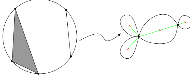
FIGURE 10. A tree of circles
