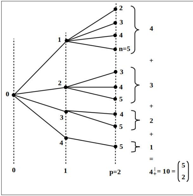
FIGURE 1. This figure represents the intellectual path from the binomial coefficient \binom{5}{2} to the termial of 4, through a classical tree view. Here, only the energy level m_1 is represented, which is sufficient, because one only has 2 energy levels, not more.
