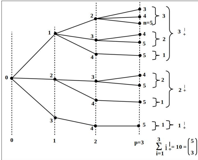
FIGURE 2. This figure represents the intellectual path from the binomial coefficient \binom{5}{3} to a sum of termials, a kind of “termial of termials” or a 2^{nd} termial. From now, one can generalize to the 3^{rd} termial, the 4^{th} termial, etc.
