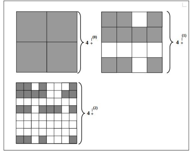
FIGURE 3. This figure tries to convert p^{th} termirial of 4 into fractal figures, for p=0 , p=1 and p=2 . Only the grey squares are counted.
