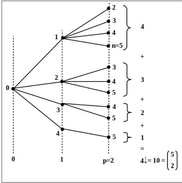
FIGURE 1. This figure represents the intellectual path from the binomial coefficient \binom{5}{2} to the termiral of 4, through a classical tree view. Here, only the energy level m_1 is represented, which is sufficient, because one only has 2 energy levels, not more.
