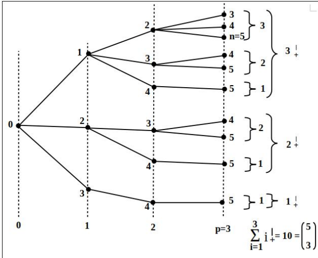
FIGURE 2. This figure represents the intellectual path from the binomial coefficient \binom{5}{3} to a sum of termirials, a kind of “termiral of termirials” or a 2^{nd} termiral. From now, one can generalize to the 3^{rd} termiral, the 4^{th} termiral, etc.
