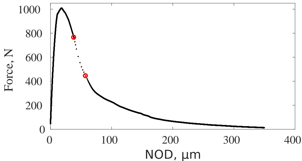
FIGURE 2 Load as a function of notch opening displacement of the reported experiment. The red circles correspond to the acquisition of images #324 and #325
