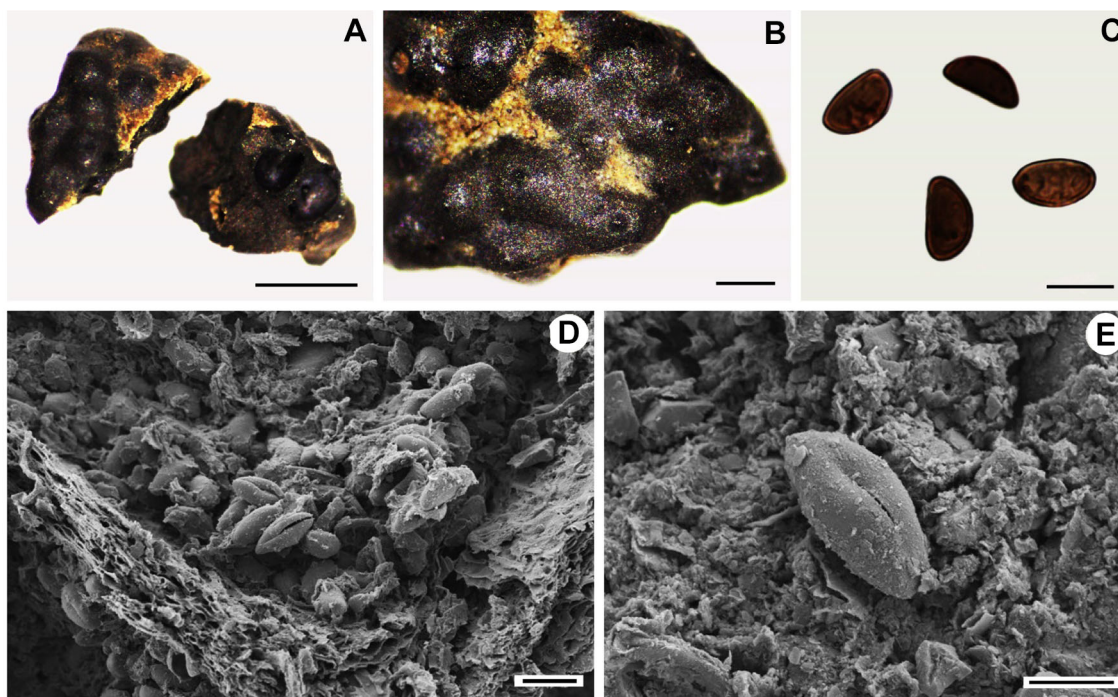
Fig. 3 Jackrogersella cohaerens (Specimen Fo2-1): a Stromata. b Ostioles. c Ascospores by light microscopy. d, e SEM images of ascospores. Scale bars: a 1000 \mu\text{m} , b 200 \mu\text{m} , c, d 10 \mu\text{m} , e 5 \mu\text{m}
