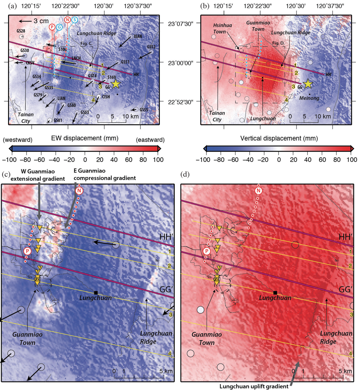
Fig. 2. (a) (b) Overview of east-west and vertical coseismic displacements determined from InSAR on Sentinel-1A images and GPS (black arrows) (Huang et al. 2016a). Yellow star shows the Meinong earthquake epicenter. Black lines are reported active faults from Taiwan Central Geological Survey. Yellow and pink lines correspond to transects shown in Fig. 3 and to geological cross-sections, respectively. Red and blue dotted lines indicate Pitou anticline (P), Guanmiao syncline (G), Napalin anticline (N), and Shihtzuchi syncline (S). (c) (d) Zooms from (a) and (b) on the Guanmiao-Lungchuan area. Yellow triangles show sites where ground surface ruptures were found. Black lines show the path covered during field survey. For convenience, only Pitou and Napalin anticlines are shown. (Color online only)
