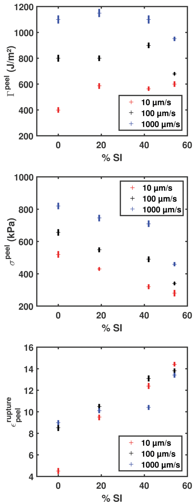
Fig. 6 Adherence energy \Gamma , average stress \sigma and maximum fibril strain \epsilon_{\text{rupture}}^{\text{peel}} in the debonding region during the peeling as a function of the diblock content and peeling velocity.
