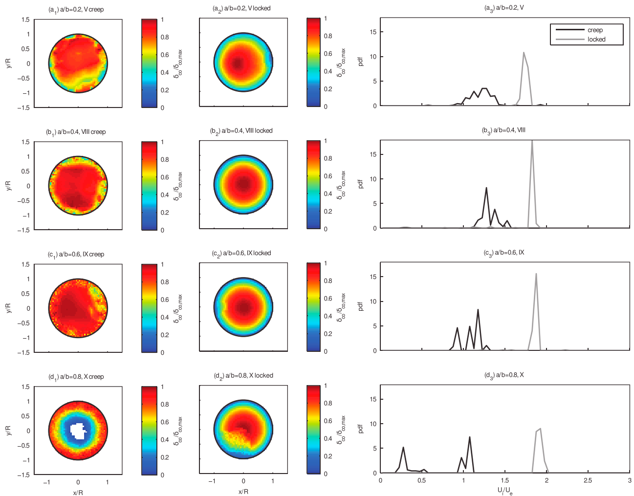
Figure 9. Same diagrams as in Figure 8, for seismicogenic patches consisting of a collection of heterogeneous asperities (structures V, VIII, IX, and X in Table 2).
