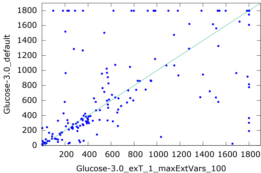
Figure 2. Scatter plot Glucose-3.0_exT_1_maxExtVars_100 vs Glucose-3.0_default The extension rule was beneficial for our solvers since they still outperformed the original solver Glucose-3.0_default for various solving time limits in term of number of solved instances. Fig. 2 shows the scatter plot comparing the original solver Glucose-3.0_default and our best performing integration namely Glucose-3.0_exT_1_maxExtVars_100 . It appears on this plot that the run time of many instances has been significantly improved: this is noticeable through the presence of many points in the upper triangle that are far from the diagonal. However there are still a number of instances where the original solver is faster.
