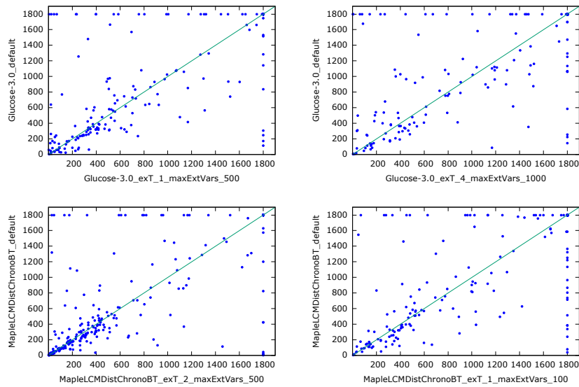
Figure 3. Scatter plots comparing some of our best integrations with the base solvers. At the left (resp. right) we have the comparison using the SC2018 (resp. SC2020) benchmarks function [10]. So it would be interesting to detect and use them instead of making new extensions with fresh variables which unnecessarily increase the formula size.
