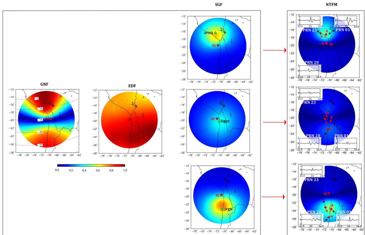
Figure 5. 2D manifestation of NTFM model in terms of GNF, EDF, SGF, and NTFM factor at IPP altitude of 350 km during the IQ earthquake. The SGF is estimated for GPS stations of iqqe , jrjn , and areq . These stations are located at the epicentral distance of ~99 km, ~409 km, and ~358 km respectively. The figure is prepared using the GMT 5.4.4 43 .
