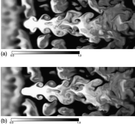
Fig. 13. Planar view of the scalar field in the Oxz plane for the turbulent simulation: (a) t = 1308.6\delta_{oi}/U ; (b) t = 1315.8\delta_{oi}/U .
