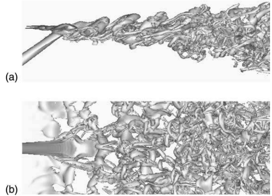
Fig. 11. Vorticity modulus iso-surface \|\omega\| = 0.5U/\delta_{oi} in the (a) Oxy plane and (b) Oxz plane.
