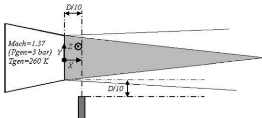
Fig. 1. Flow arrangement.
