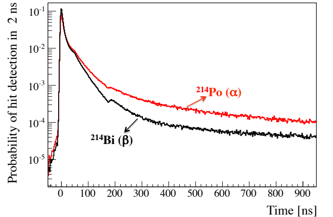
FIG. 27. The reference r_\alpha(t_n) (red) and r_\beta(t_n) (black) pulse shapes obtained by tagging the radon-correlated ^{214}\text{Bi} - ^{214}\text{Po} coincidences. The dip at 180 ns is due to the dead time on every individual electronic channel applied after each detected hit (see Section VI). The small shoulder around 60 ns is due to the light reflected on the SSS surface and on the PMTs' cathodes.
