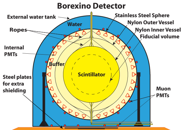
FIG. 2. The schematic view of the Borexino detector.
