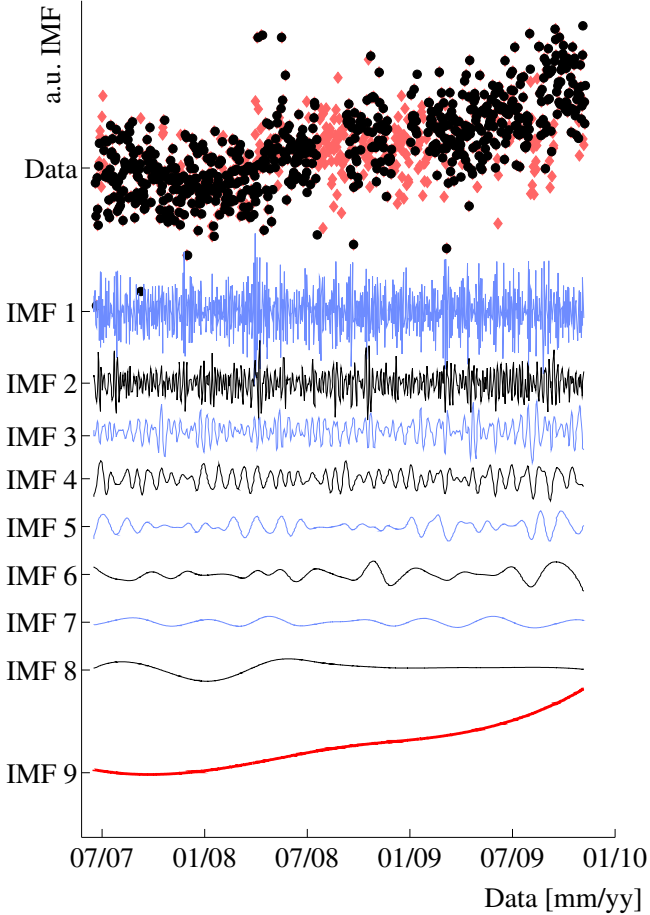
FIG. 68. A sequence of the IMF extracted from the data (black circles) plus white noise (red diamonds) by means of a sifting algorithm using 20 iterations for each one. The \text{IMF}_8 is the one used to extract the results about the seasonal modulation, The last \text{IMF}_9 , also called “trend”, is the best representation of the background variation in time.
