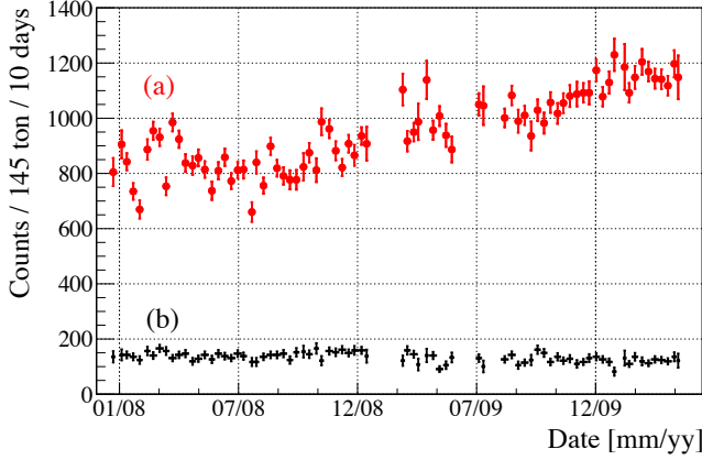
FIG. 65. Rate of events in the energy region 105 < N_{pe}^d < 380 and in the FV used in the seasonal modulation analysis as a function of time shown with 10-day binning: the red data points (a) were scaled by a constant factor. For comparison, the black plot (b) shows the count rate due to external \gamma s which is stable in time since it is not correlated with the changes of the IV shape.
