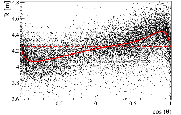
FIG. 19. R - \cos(\theta) distribution of the events in the energy region 800 - 900 keV from November 2007 used for the IV shape reconstruction. The best-fit vessel shape is shown in a solid red line. The dotted red line represents the nominal spherical vessel with R = 4.25 m.
