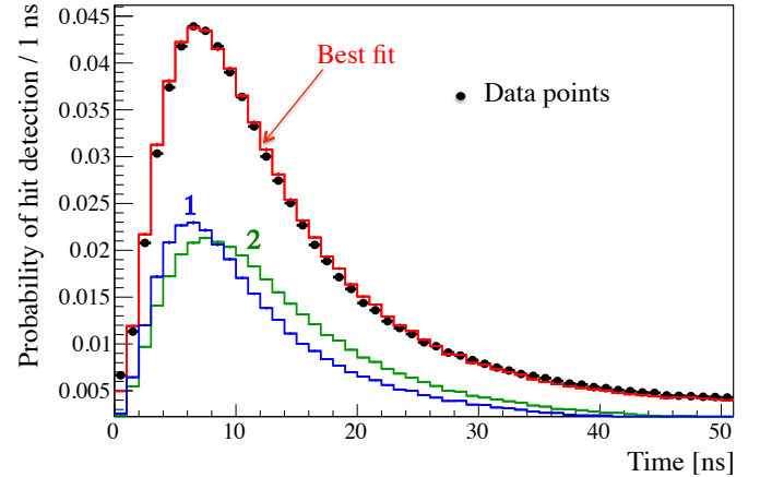
FIG. 43. Reconstructed photon emission times for ^{11}\text{C} events. The data (black points) has been fitted to the ^{11}\text{C} Monte Carlo shapes without (1-blue) and with (2-green) ortho-positronium formation (mean-life of 3.1 ns); the relative weights of these two shapes were left free in the fit. The best fit, the sum of the two MC-shapes, is shown red.
