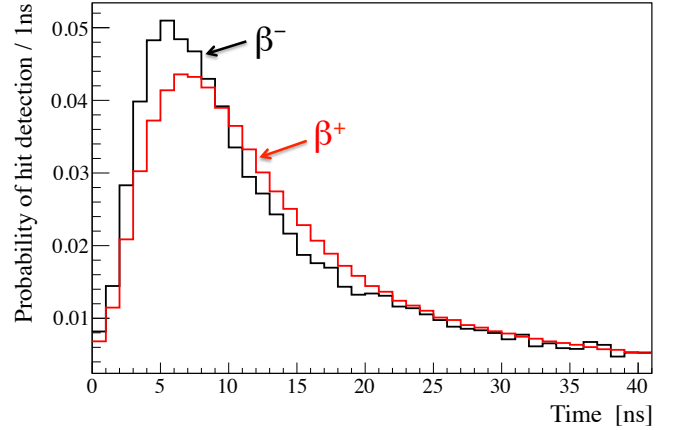
FIG. 42. Reconstructed photon emission times relative to the start time of the cluster: ^{214}\text{Bi} ( \beta^- ) events with 425 < N_h < 475 identified by a ^{214}\text{Bi} - ^{214}\text{Po} fast coincidence tag (black) and ^{11}\text{C} ( \beta^+ ) events tagged by the TFC (red).
