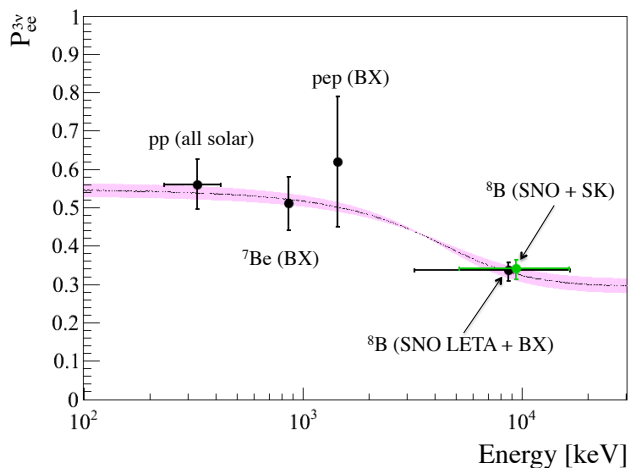
FIG. 84. Electron neutrino survival probability as a function of neutrino energy according to MSW-LMA model. The band is the same as in Fig. 83, calculated for the production region of {}^8\text{B} solar neutrinos which represents well also other species of solar neutrinos. The points represent the solar neutrino experimental data for {}^7\text{Be} and pep mono-energetic neutrinos (Borexino data), for {}^8\text{B} neutrinos detected above 5000 keV of scattered-electron energy T (SNO and Super-Kamiokande data) and for T > 3000 keV (SNO LETA + Borexino data), and for pp neutrinos considering all solar neutrino data, including radiochemical experiments.
