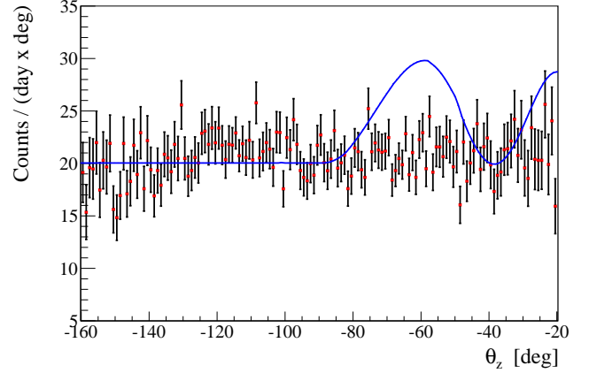
FIG. 58. Normalized \theta_z -angle distribution of the events in the {}^7\text{Be}-\nu energy window and reconstructed within the enlarged FV. The effect of the Earth elliptical orbit has been removed. The fit with a flat straight line yields \chi^2/\text{NDF} = 141.1/139 . The blue solid line shows the expected effect with the LOW solution \Delta m_{12}^2 = 1.0 \cdot 10^{-7} \text{ eV}^2 and \tan \theta_{12}^2 = 0.955 .
