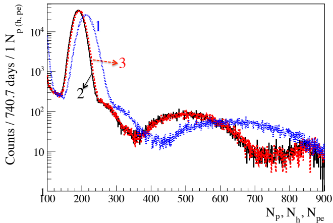
FIG. 33. Final spectra for all events in the {}^7\text{Be}-\nu FV passing all selection cuts, shown in three different energy estimators: N_{pe} (1-dotted blue), N_p (2-solid black), and N_h (3-dashed red).
