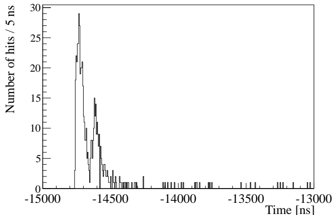
FIG. 30. Example of an event with N_{peak} = 2 . The horizontal axis shows the time difference of each hit with respect to trigger signal, so the absolute values have no physical meaning.
