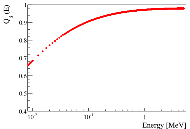
FIG. 8. The quenching factor Q_\beta(E) calculated from Eq. 7 with the Borexino quenching parameter kB = 0.011 \text{ cm/MeV} .
