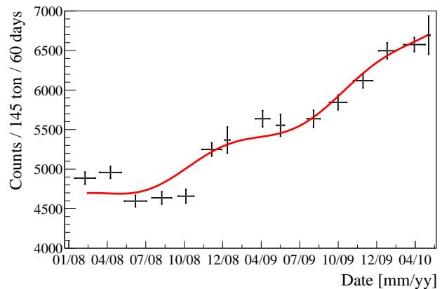
FIG. 63. Results obtained with rate analysis. The continuous line is the curve of Eq. 84. The data are grouped in bins of 60 days.
