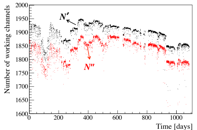
FIG. 10. The number N' (black) and N'' (red) of available channels for the computation of N_h / N_p and N_{pe} energy estimators, respectively, as a function of time starting from May 16 th , 2007 (day 0). The slow decrease is due to the PMT mortality, while the sudden changes are due to the failure/repair of the electronics.
