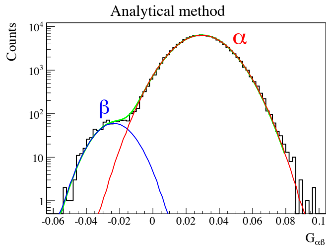
FIG. 36. Example of \alpha - \beta statistical subtraction with the analytical method for events in the energy range 200 < N_{pe}^d < 205 . The blue and red lines show the individual Gaussian fits to the Gatti parameter distributions for the \beta and \alpha components, respectively, while the green line is the total fit.
