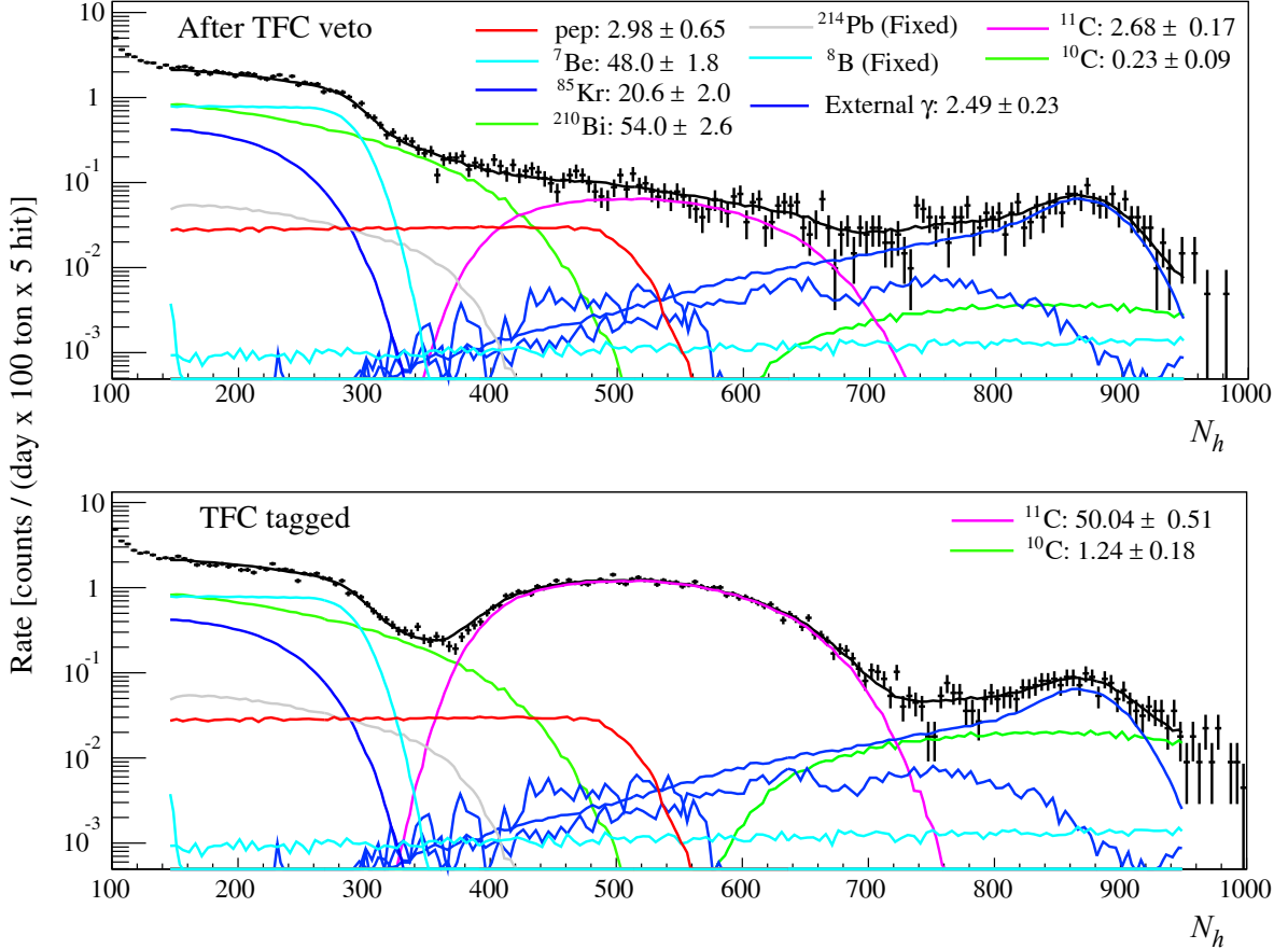
FIG. 71. Energy spectra and the best-fit results performed on the N_h energy estimator in the pep and CNO neutrino analysis. The top panel shows the best fit to the TFC-subtracted spectrum, while the bottom one presents the fit to the complementary, TFC-tagged events. The best-fit values for the rates of the species included in the fit are shown in the legend. Units are cpd/100 ton.
