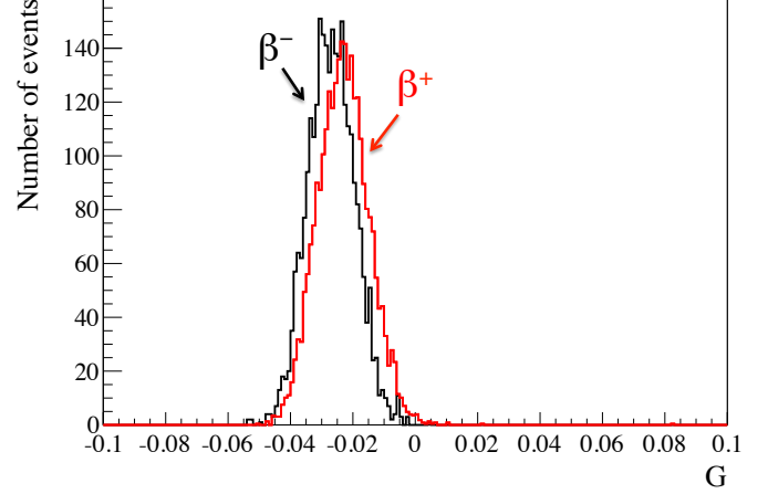
FIG. 29. The distribution of the G_\beta^- parameter (black) obtained from ^{214}\text{Bi} ( \beta^- ) events and of the G_\beta^+ parameter (red) obtained from ^{11}\text{C} ( \beta^+ ) events.
