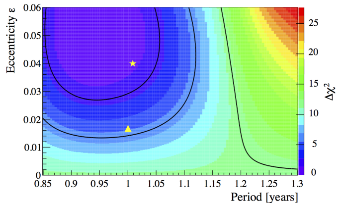
FIG. 64. The results obtained via the fit of the rate-versus-time distribution shown in Fig. 63: a \Delta\chi^2 ( \Delta\chi^2 = \chi_{R_{min}}^2 - \chi_{R_{xy}}^2 ) map (vertical axis) as a function of eccentricity \varepsilon and period. The yellow star indicates the best-fit results, while the yellow triangle the expected values. Confidence contours of 1, 2, and 3\sigma are indicated with black solid lines.
