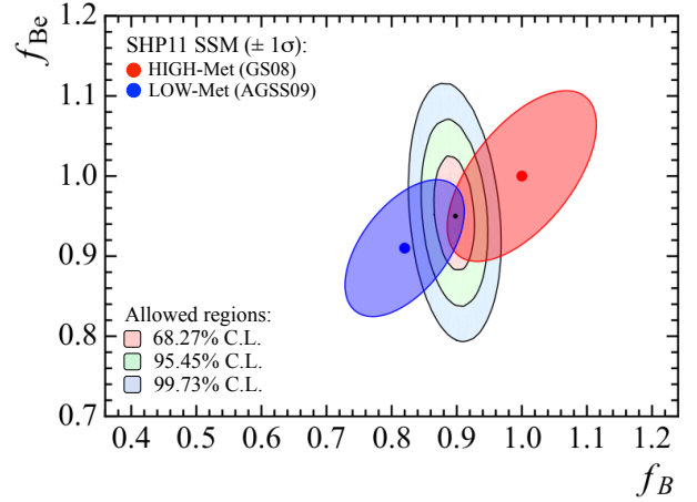
FIG. 82. The 1\sigma theoretical range of high (red) and low (blue) metallicity Standard Solar Model for f_{\text{Be}} and f_{\text{B}} , compared to the 1\sigma (light pink), 2\sigma (light green), and 3\sigma (light blue) allowed regions by the global analysis of solar-with-Borexino plus KamLAND results. The theoretical correlation factors are taken from [87].
