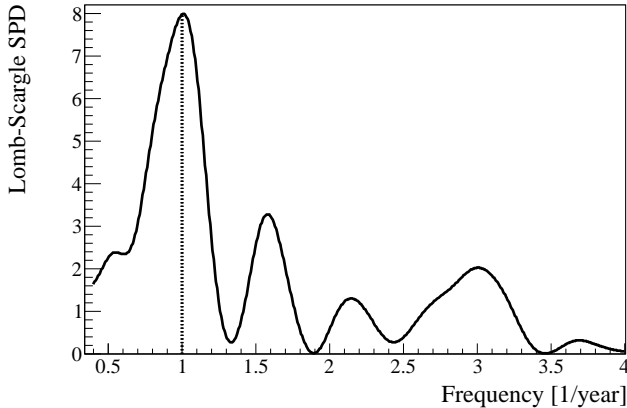
FIG. 66. Lomb-Scargle periodogram for the red data points marked (a) in Fig. 65 after the subtraction of the exponential trend due to the ^{210}\text{Bi} contamination. The Spectral Power Density at 1-year is 7.961, as indicated by the vertical line.
