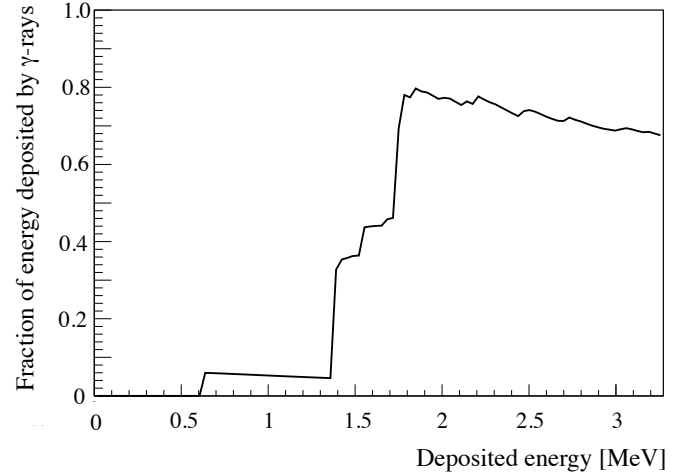
FIG. 44. Average fraction of the energy deposited by ^{214}\text{Bi} decays in the form of \gamma -rays. For deposited energy below 1400 keV, only less than 5% of the energy is due to \gamma -rays. Therefore, low-energy ^{214}\text{Bi} decays are a sample of mostly pure \beta^- decays.
