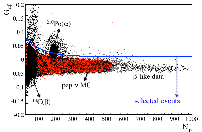
FIG. 35. The distribution of the Gatti G_{\alpha\beta} parameter as a function of energy ( N_p variable). The continuous (blue) line shows the energy dependent cut; it removes all the events with G_{\alpha\beta} above the line. The (red) points enclosed within the dashed line show the G_{\alpha\beta} distribution for MC-simulated pep - \nu 's; these events are an example of true \beta events with a spectrum extending over a sufficiently large energy range. The \beta events are not affected by this cut, while, on the contrary, this cut removes a large fraction of the \alpha events, as those from the {}^{210}\text{Po} decay.
