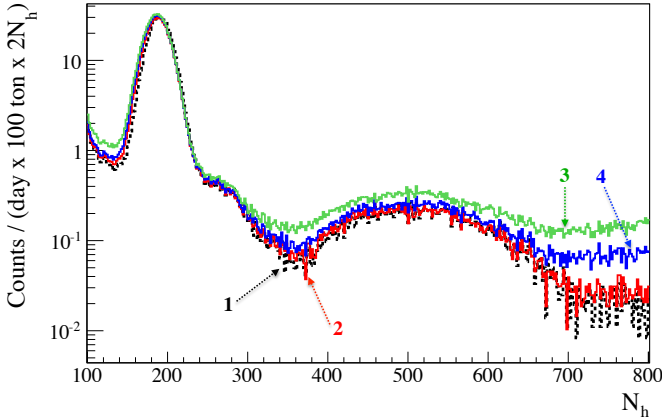
FIG. 57. Energy spectra ( N_h ) during the day time in different volumes. The two curves showing the lowest count rate and almost superimposed have been obtained selecting events within the standard FV used for the {}^7\text{Be}-\nu rate analysis (1 - black dotted line) and within a sphere of 3 m radius (2 - red solid line). The curve with the highest count rate (3 - green) shows the events selected within a 3.5 m radius sphere while the curve with the intermediate count rate (4 - blue) refers to a 3.3 m radius sphere.
