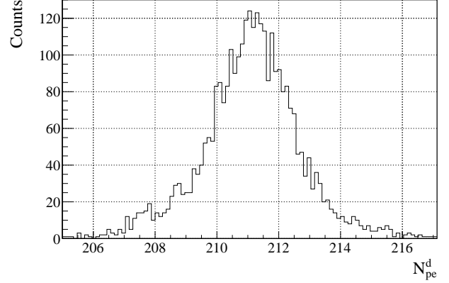
FIG. 61. Energy distribution of the {}^{210}\text{Po}(\alpha) peak (expressed in N_{pe}^d estimator) in the FV used for the {}^7\text{Be}-\nu annual modulation analysis.
