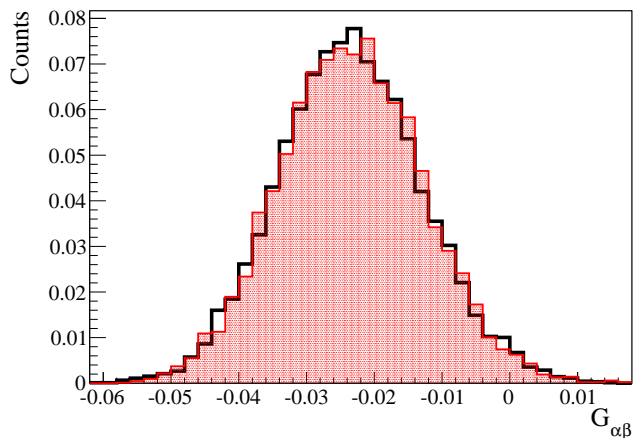
FIG. 51. The G_{\alpha\beta} variable for the {}^{85}\text{Sr} \gamma -calibration source placed at the location (x, y, z) = (0, 0, 3) m, for measured (black line) and Monte Carlo simulated (red filled area) events.
