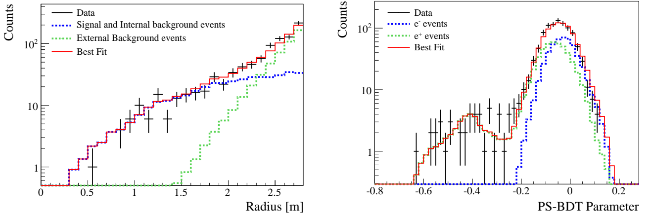
FIG. 73. Left: Radial distribution of events in the energy range N_h = 500 - 900 (black data points) and the best fit (solid-red line) obtained performing the multivariate fit with the N_h energy estimator. The y -axis scale is logarithmic. A similar and statistically consistent result is obtained using the variable N_{pe}^d . Right: Distribution of the PS-BDT parameter for events in the energy range 450 - 900 N_{pe}^d (black data points) and the best fit (solid-red line) obtained performing the multivariate fit with the variable N_{pe}^d . The scale is logarithmic. Similar and consistent results are obtained with N_h variable.
