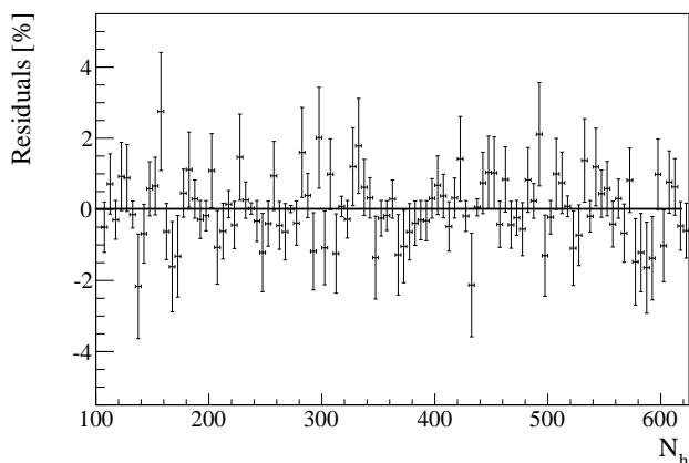
FIG. 55. Typical example of the distribution of the residuals of the fit. This plot corresponds to the fit shown in Fig. 54.
