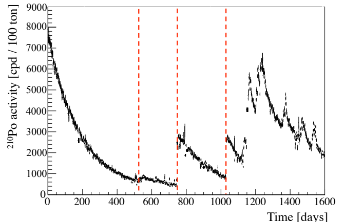
FIG. 24. {}^{210}\text{Po} count rate in the FV used in the {}^7\text{Be}-\nu rate analysis as a function of time. The various increases are due to the IV-filling operations shown by the three vertical lines (Section II.1) and due to the tests of the purification methods (details in text).
