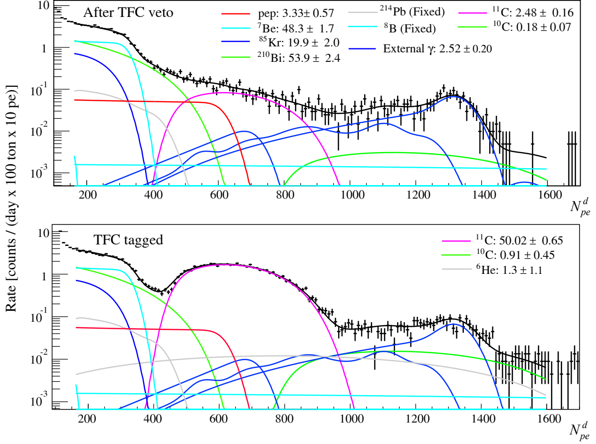
FIG. 72. Energy spectra and the best-fit results performed on the N_{pe}^d energy estimator in the pep and CNO neutrino analysis. The top panel shows the best fit to the TFC-subtracted spectrum, while the bottom one presents the fit to the complementary, TFC-tagged events. The best-fit values for the rates of the species included in the fit are shown in the legend. Units are cpd/100 ton.
