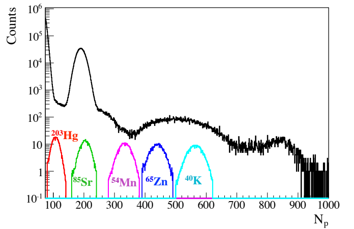
FIG. 34. Final spectrum for all events passing all selection cuts is shown in N_p variable (black) with respect to the \gamma -sources calibration spectra: {}^{203}\text{Hg} (red), {}^{85}\text{Sr} (green), {}^{54}\text{Mn} (magenta), {}^{65}\text{Zn} (blue), and {}^{40}\text{K} (cyan). The calibration peaks are all normalized to an area of 500.
