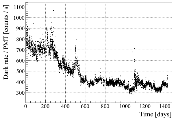
FIG. 4. Mean dark-noise rate per PMT in counts per second as a function of time starting from May 16 th , 2007 (day 0).
