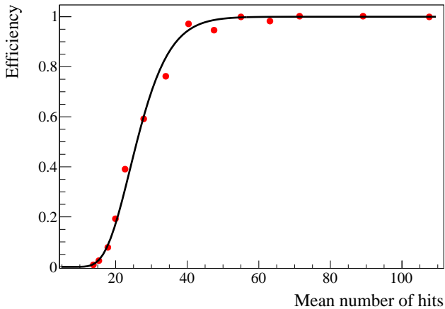
FIG. 6. The trigger efficiency as a function of the average number of detected PMT hits. For each point, the average number of hits was obtained from the calibration shown in Fig. 5. The fit function is an error function with standard deviation computed assuming exact Poisson statistics. The fit mean value is 25.7, in a very good agreement with the nominal triggering threshold of K = 25 .
