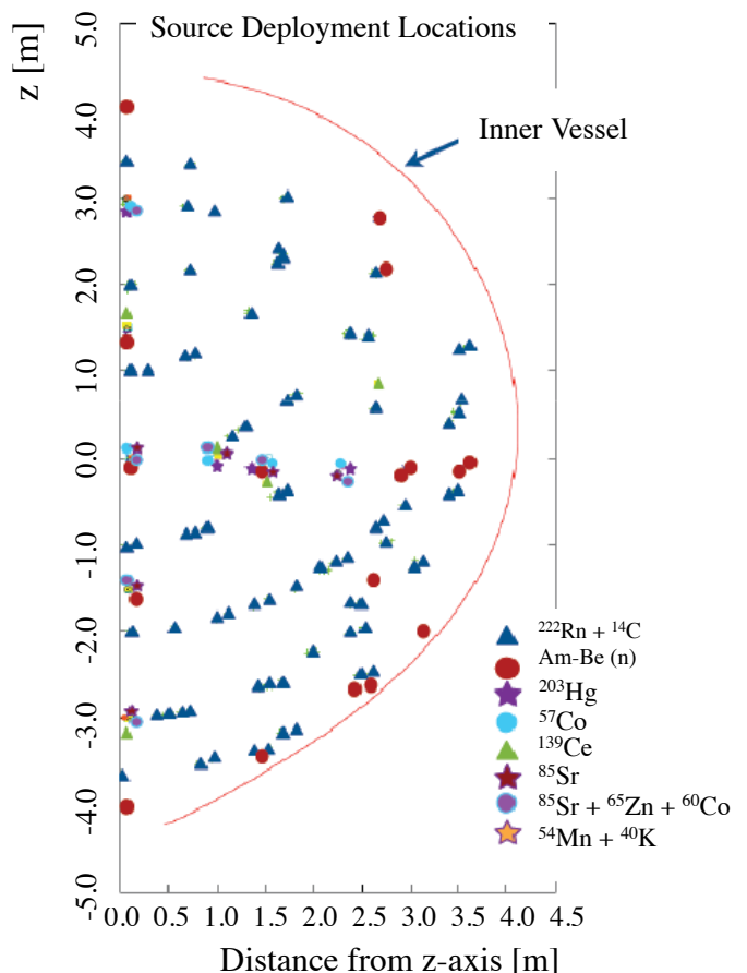
FIG. 9. Position of the various radioactive sources deployed in the scintillator and used to calibrate the Borexino detector.
