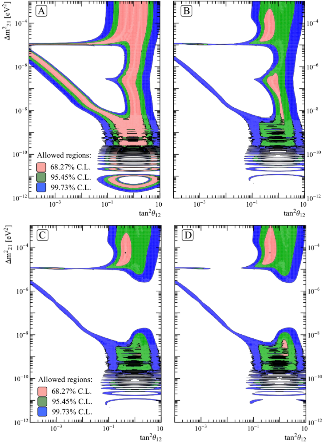
FIG. 78. The Borexino data analysis in the \tan^2 \theta_{12} - \Delta m_{21}^2 space. Allowed regions (NDF = 2) at 68.27% C.L. (pink), 95.45% C.L. (green), and 99.73% C.L. (blue). Panel A: impact of the Borexino {}^7\text{Be}-\nu rate measurement. Panel B: the combined analysis of Borexino measurements of {}^7\text{Be}-\nu and {}^8\text{B}-\nu rates. Panel C: the impact of {}^7\text{Be}-\nu and {}^8\text{B}-\nu rates together with the {}^7\text{Be}-\nu day–night asymmetry results. Panel D: the global impact of all the Borexino measurements to date, including the pep-\nu rate.
