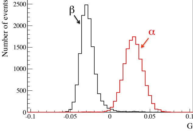
FIG. 28. The distribution of G_\alpha (red) and G_\beta (black) (see Eq. 28) for events obtained by tagging the radon correlated ^{214}\text{Bi} - ^{214}\text{Po} coincidences.
