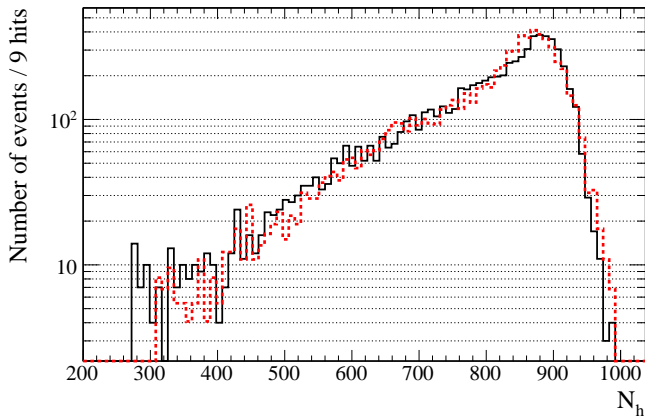
FIG. 15. Comparison between the energy spectra ( N_h energy estimator) for events from the external ^{228}\text{Th} / ^{208}\text{Tl} source calibration data (black solid line) and from the 2610 keV simulated external \gamma rays (red dotted line), reconstructed within 3 m from the detector center. The \chi^2/\text{NDF} between the two histograms is \simeq 1.2 . The source is positioned in the upper hemisphere; a similar result is obtained for the lower one.
