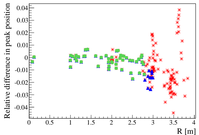
FIG. 49. The relative difference \frac{N_h(\text{MC}) - N_h(\text{data})}{N_h(\text{data})} as a function of the radial position R of the ^{214}\text{Po} \alpha peak from the radon calibration source. Blue triangles: ^7\text{Be}-\nu FV, green circles: pep-\nu FV, red stars: outside both FVs.
