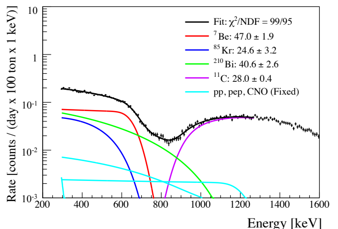
FIG. 53. Example of fit of the energy spectrum obtained using the analytical method with \alpha - \beta statistical subtraction. The fit was done using the N_{pe}^d energy estimator. After the fit, the horizontal axis was converted into energy scale in keV. The values of the best-fit parameters, the rates of individual species, are given in cpd/100 ton.
