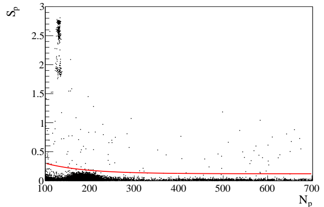
FIG. 31. An example of the application of the S_p energy-dependent cut (see Eq. 39) indicated by the solid red line on a sample of events which are not tagged as muons and which are reconstructed in the ^7\text{Be} -FV. The events having the S_p variable above the value indicated by the line are excluded from the data set. Clearly, the cluster at energies of N_p \sim 130 with S_p > 1.7 is due to anisotropic noise events.
