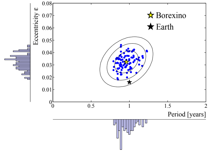
FIG. 70. Blue circles show the eccentricities and periods obtained with the EMD method with 100 \text{IMF}_8 's (see Fig. 69). The projections shown on the vertical and horizontal axis are well described by Gaussian curves. The solid-black line of Fig. 69 is represented by the yellow star in the middle of 1, 2, and 3\sigma C.L. contours. The black star represents the expectations. The measured period is in perfect agreement with 1 year, while the eccentricity is compatible within 3\sigma .
