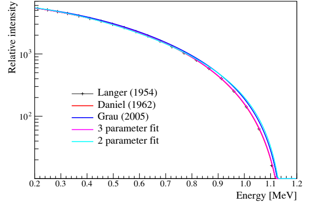
FIG. 77. Comparison between the ^{210}\text{Bi} energy spectrum measured using the magnetic spectrometer [79] (crosses, labeled as Langer (1954)) with spectra obtained using different correction factors: those calculated in [80] (red curve labeled as Daniel (1962)) and in [81] (blue curve labeled as Grau (2005)). Also shown are the fit to the Langer data according to Eq.88 with all the three parameters and with b=0 .
