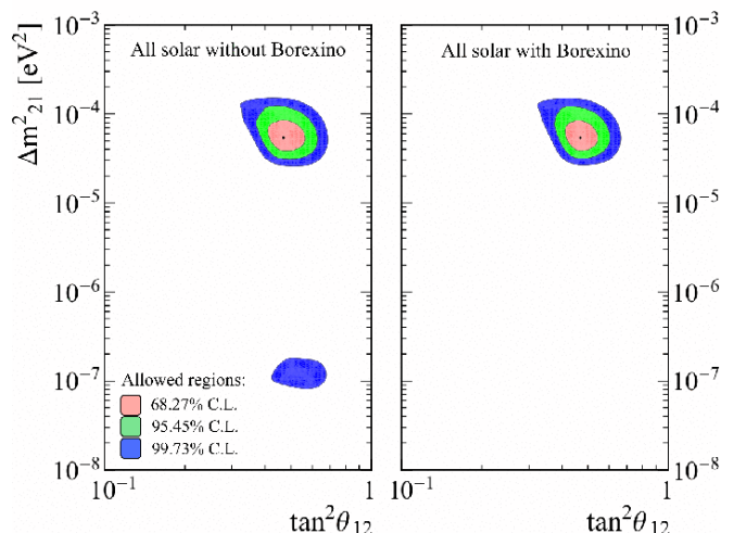
FIG. 80. Allowed regions (NDF = 3) of the space of parameters at 68.27% C.L. (pink), 95.45% C.L. (green), and 99.73% C.L. (blue) by the solar-without Borexino (left panel) and solar-with Borexino (right panel) data set.
