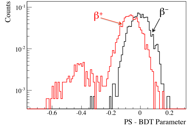
FIG. 45. Distributions of the PS-BDT parameter for the test samples of \beta^- (black) and \beta^+ (red) events as described in the text.
