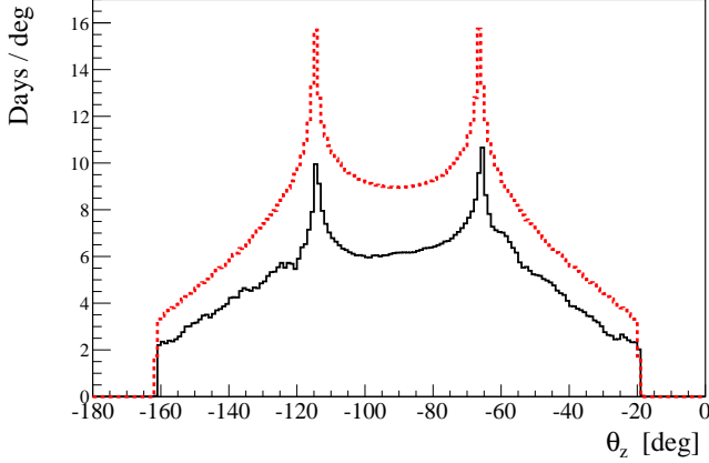
FIG. 56. The experimental exposure function (black continuous line) and the ideal exposure function (red dotted line) corresponding to 3 years of data taking without interruptions at LNGS, as functions of the \theta_z angle (1 deg/bin). The interval from -180^\circ to -90^\circ corresponds to day (360.25 days) and the one from -90^\circ to 0^\circ to night time (380.63 days). We recall that at LNGS latitude the Sun is never at the zenith.
