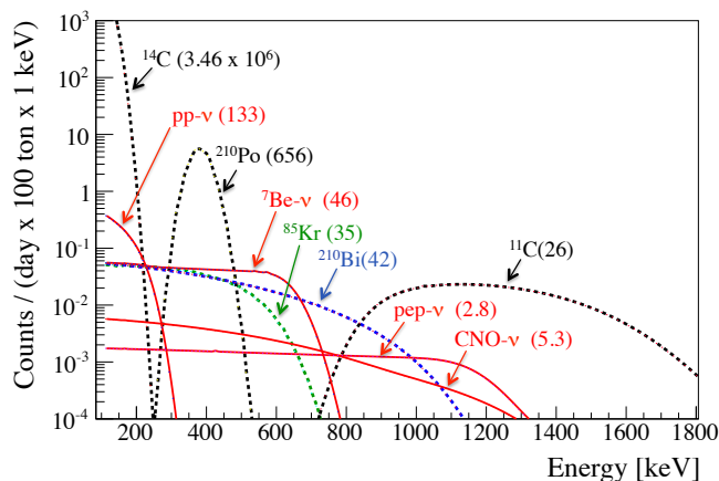
FIG. 20. Calculated energy spectra due to solar neutrinos (shown as continuous red line) and of the main background components (dotted lines). The realistic Borexino energy resolution is included. The rates are fixed at the values shown in parenthesis and given in units of cpd/100 ton.
