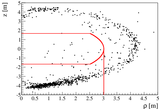
FIG. 26. Distribution of the ^{212}\text{Po} events (from ^{212}\text{Bi} - ^{212}\text{Po} coincidences) in the z - \rho plane from May 2007 to May 2010. The solid red line indicates the FV used in the ^7\text{Be}-\nu analysis.
