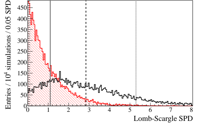
FIG. 67. Distributions of the Lomb-Scargle Spectral Power Density (SPD) at frequency corresponding to 1 year for 10^4 simulations of a 7% solar-neutrino annual flux modulation with realistic background (solid black line) and the same number of white-noise simulations of background without any seasonally-modulated signal (red area). Indicated with vertical lines are the sensitivity thresholds of 1\sigma (solid), 2\sigma (dashed), and 3\sigma (dotted) C.L. with corresponding detection probabilities of 81.62, 43.54, and 11.68%, respectively. The detected SPD(1\text{ year}) = 7.961 (see Fig. 66) represents an evidence of the annual-modulation signal with a significance higher than 3\sigma ; our chance of detecting the annual modulation at this level of significance is 11.68%.
