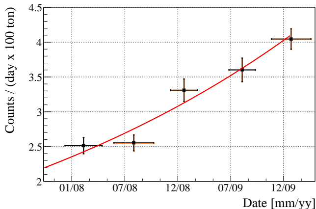
FIG. 23. Count rate R(t) in the energy region from 390 < N_{pe}^d < 450 in the FV used for the {}^7\text{Be}-\nu annual modulation analysis from the beginning of the year 2008 until the middle of year 2010. This region is dominated by the {}^{210}\text{Bi} contribution. The red line is a fit according to Eq. 22.
