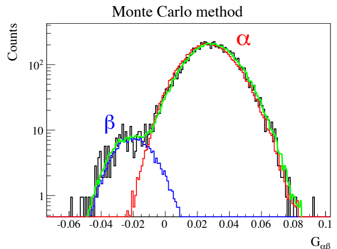
FIG. 37. Example of \alpha - \beta statistical subtraction with the Monte Carlo method for events in the energy range 168 < N_h < 170 . The plot shows the Gatti parameter of the data (black) and the fit (green) aiming to separate the \alpha (red) and \beta (blue) contributions. In comparison to analytical method demonstrated in Fig. 36, the blue \beta and \alpha shapes are Monte Carlo shapes which are not Gaussian. Details in text.
