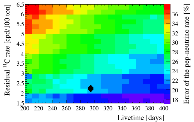
FIG. 38. Prediction of the sensitivity to the pep - \nu interaction rate measurement ( z -axis) as a function of the residual ^{11}\text{C} rate ( y -axis) and the effective live-time ( x -axis) obtained by fitting the MC-simulated data. The color z -axis is expressed as the uncertainty (%) on the pep - \nu interaction rate returned by the fit. We recall that the ^{11}\text{C} rate measured without applying the TFC subtraction is (28.5 \pm 0.2(\text{stat}) \pm 0.7(\text{sys})) cpd/100 ton. The black diamond corresponds to the TFC-subtracted spectrum used in the analysis (see Fig. 40).
