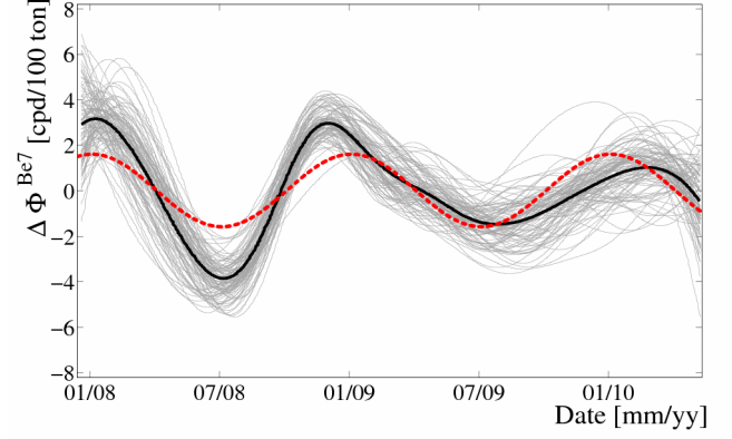
FIG. 69. Set of 100 intrinsic mode functions \text{IMF}_8 extracted after the addition of dithering (grey lines). The black-solid line is their average and the dashed-red line is the annual modulation from Eq. 84. The number of the IMF is the expected one for the annual frequency of \nu_{\text{year}} = 0.00274 [d^{-1}] .
