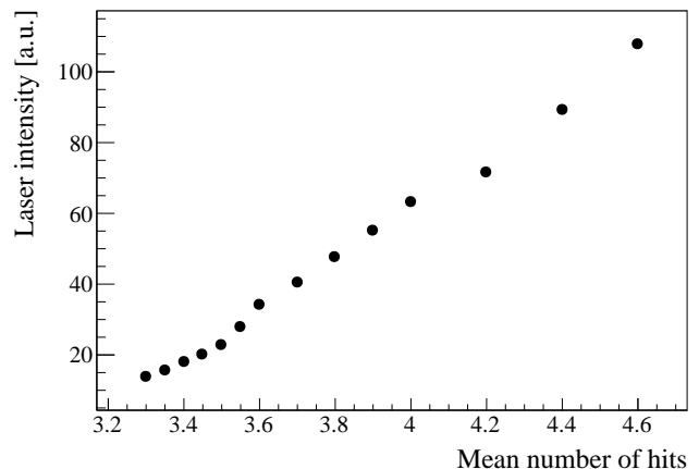
FIG. 5. Top: examples of the distributions of the number of PMT hits for three laser intensities; Bottom: relation between the average number of PMT hits detected by Borexino Inner Detector and the laser intensity. These calibration values, which are approximately, but not exactly, linear, were used to compute the detection efficiency shown in Fig. 6.
