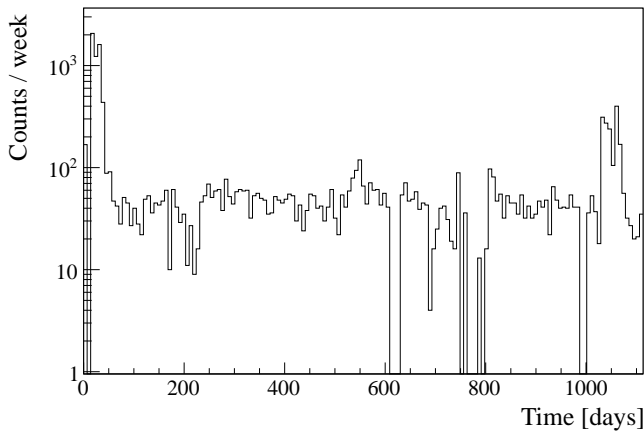
FIG. 21. Number (counts/week) of ^{214}\text{Bi} - ^{214}\text{Po} coincidences detected in the whole scintillator volume as a function of time starting from May 16 th , 2007 (day 0). The spikes are due to the filling operations.
