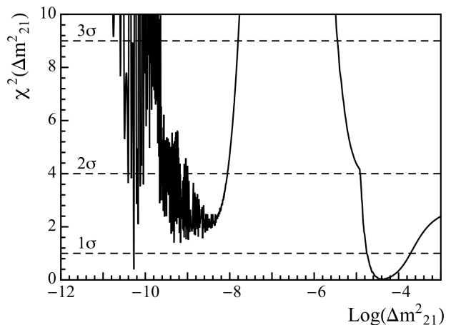
FIG. 79. The \chi^2 -profile of the \Delta m_{21}^2 parameter in the Borexino results analysis. The dashed lines indicate the 1\sigma [ \chi^2(\Delta m_{21}^2)=1 ], 2\sigma [ \chi^2(\Delta m_{21}^2)=4 ], and 3\sigma [ \chi^2(\Delta m_{21}^2)=9 ] levels. The MSW-LOW region ( 10^{-8} \text{ eV}^2 < \Delta m_{21}^2 < 10^{-6} \text{ eV}^2 ) is ruled out at more than 8.5\sigma .
