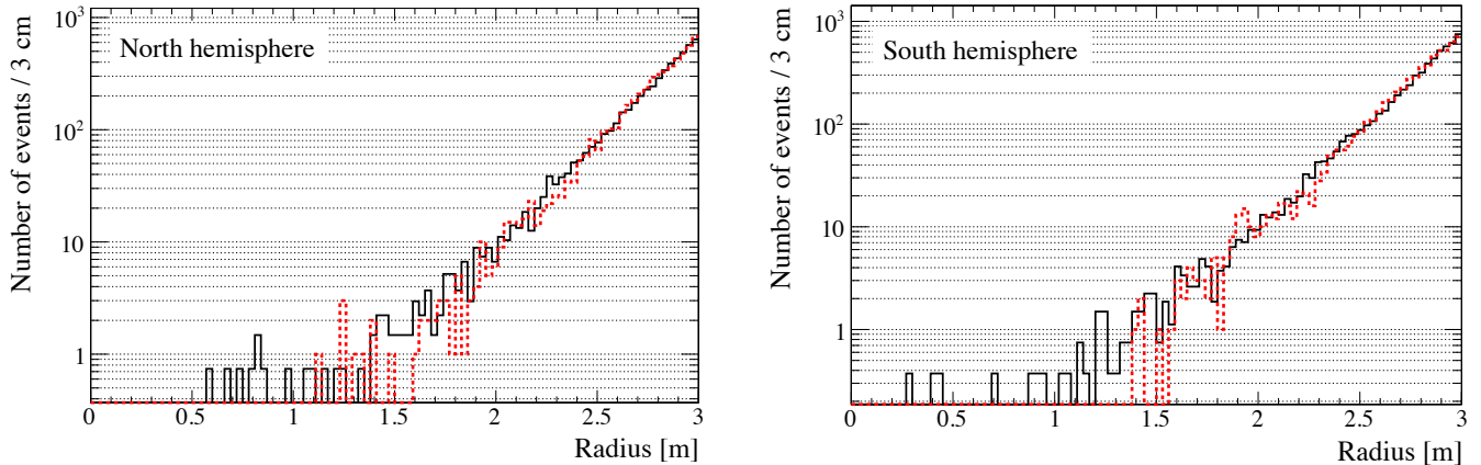
FIG. 16. Comparison between the reconstructed radius of events with energy N_h > 400 from the external ^{228}\text{Th} / ^{208}\text{Tl} source calibration data (black solid line) and from the 2610 keV simulated external \gamma rays (red dotted line), reconstructed within 3 m from the detector center. The left and right plots show examples for a source position in the upper/north and lower/south hemispheres, respectively. The \chi^2/\text{NDF} between the two histograms (Monte Carlo and data) is in the range 0.8 – 0.9.
