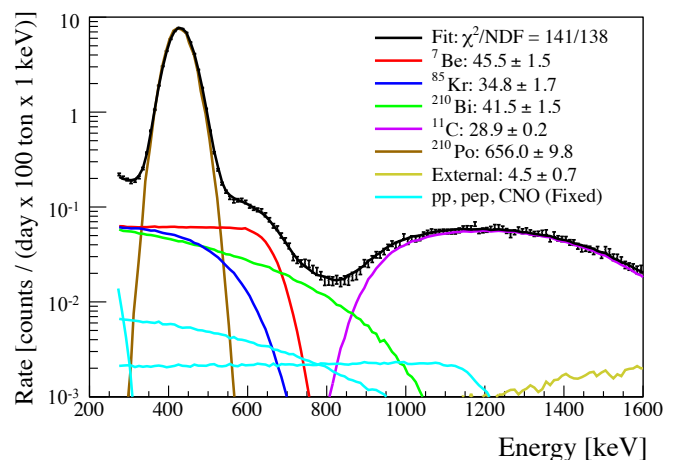
FIG. 52. Example of fit of the energy spectrum obtained using the Monte Carlo method without \alpha - \beta statistical subtraction. The fit was done using the N_h energy estimator. After the fit, the horizontal axis was converted into energy scale in keV. The values of the best-fit parameters, the rates of individual species, are given in cpd/100 ton.
