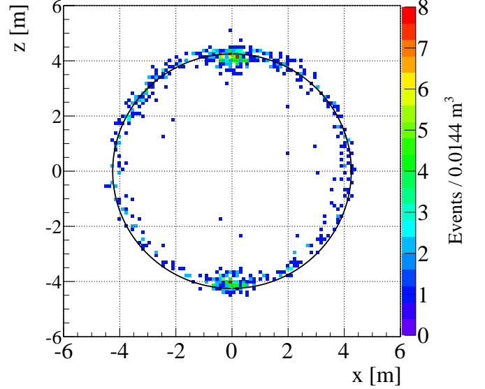
FIG. 18. z - x distribution ( |y| < 0.5 m) of the events in the energy region 800 - 900 keV, which are mainly due to {}^{210}\text{Bi} contaminating the IV surface. The color axis represents the number of events per 0.0144 \text{ m}^3 in a pixel of 0.12 \text{ m} \times 1.00 \text{ m} \times 0.12 \text{ m} ( x \times y \times z ). This spatial distribution reveals the IV shift and deformation with respect to its nominal spherical position shown in solid black line.
