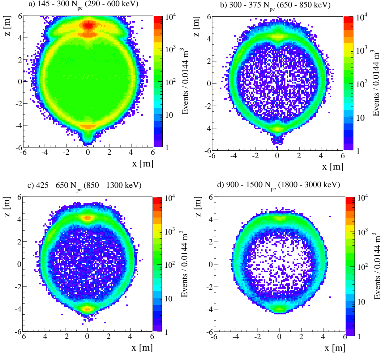
FIG. 14. Spatial distribution (in the x - z plane, |y| < 0.5 m) of all reconstructed events (besides muons) in different energy regions. The color axis represents the number of events per 0.0144 \text{ m}^3 in a pixel of 0.12 \text{ m} \times 1.00 \text{ m} \times 0.12 \text{ m} ( x \times y \times z ). a) ^{210}\text{Po} peak region: 145 - 300 N_{pe} (290 - 600 keV), b) ^7\text{Be} shoulder: 300 - 375 N_{pe} (650 - 850 keV), c) ^{11}\text{C} energy region: 425 - 650 N_{pe} (850 - 1300 keV), d) ^{208}\text{Tl} peak region: 900 - 1500 N_{pe} (1800 - 3000 keV). Events occurring outside the IV ( R = 4.25 m), near the top end-cap ( z = 4.25 m), most clearly seen in the low-energy region shown in a) plot, are due to the small leak of scintillator from the IV to the buffer region (Section II.1).
