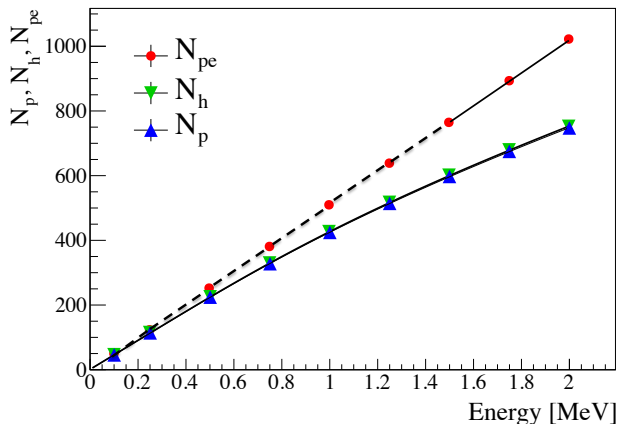
FIG. 50. The energy estimators N_p , N_h , and N_{pe} versus energy for \beta events uniformly generated in the {}^7\text{Be} -FV as obtained with the Monte Carlo simulation.
