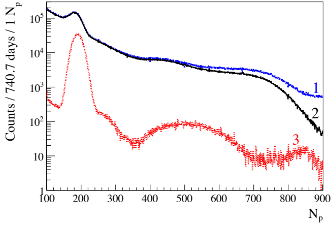
FIG. 32. Effect of selection cuts on the raw spectrum in the N_p variable (marked 1 and shown in blue). The black spectrum (marked 2) shows the effect of the muon and muon daughter cut. The shape of the final N_p spectrum (marked 3 and shown in red) is dominated by the effect of the {}^7\text{Be}-\nu FV cut. The effect of other cuts described in Section XIII.1 is important at the level of fit, but cannot be appreciated visually.
