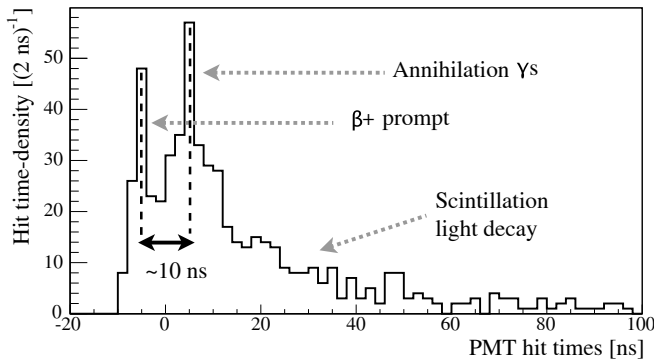
FIG. 41. Hit-emission time profile of a single event due to \beta^+ decay, where the positron deposits its kinetic energy (first peak) and then forms ortho-positronium. The ortho-positronium exists for \sim 10 ns before the positron annihilates with a bulk electron to produce \gamma -rays (second peak). The PS-BDT value (Fig 45) of this cluster is -0.44.
