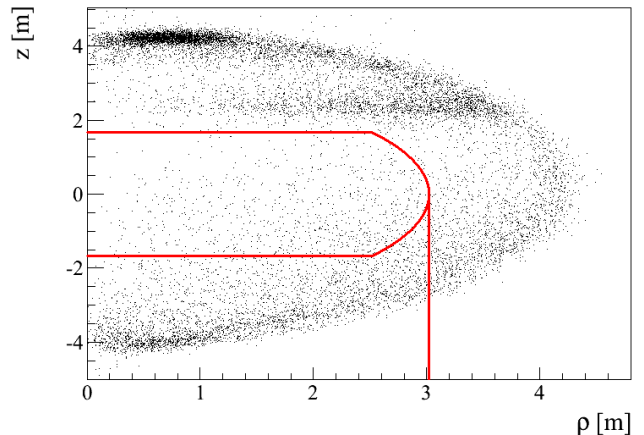
FIG. 22. Spatial distribution of the ^{214}\text{Po} events (from ^{214}\text{Bi} - ^{214}\text{Po} coincidences) in the z - \rho plane from May 2007 to May 2010. The solid red line indicates the FV used in the ^7\text{Be} - \nu analysis. The layer of events in the upper hemisphere is outside this volume and corresponds to the increased rate of radon at the beginning of data taking (see Fig. 21).
