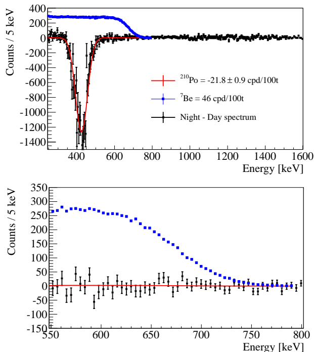
FIG. 59. Difference of the night and day spectra in the enlarged FV. The top panel shows an extended energy range including the region dominated by the ^{11}\text{C} background while the bottom panel is a zoom in the ^7\text{Be}-\nu energy window. The fit is performed in the ^7\text{Be}-\nu energy region (between 250 and 800 keV) with the residual ^{210}\text{Po} spectrum and the electron recoil spectrum due to the ^7\text{Be} solar neutrino interaction. The blue curve plots the ^7\text{Be}-\nu spectrum used in the fit with the amplitude \langle R \rangle = 46 cpd/100 ton. The residual ^7\text{Be}-\nu resulting from the fit is too small to be shown.
