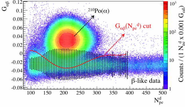
FIG. 60. G_{\alpha\beta} parameter in the FV used in the seasonal modulation analysis shown as a function of energy ( N_{pe}^d estimator). The red line indicates where the Gatti-cut was placed: in the window of (105, 380) N_{pe}^d , 66% of \beta 's survive while almost 100% of \alpha 's is rejected. Black bars represent, for different energy bins, the G_{\beta} interval covering 99.9% of \beta -events.
