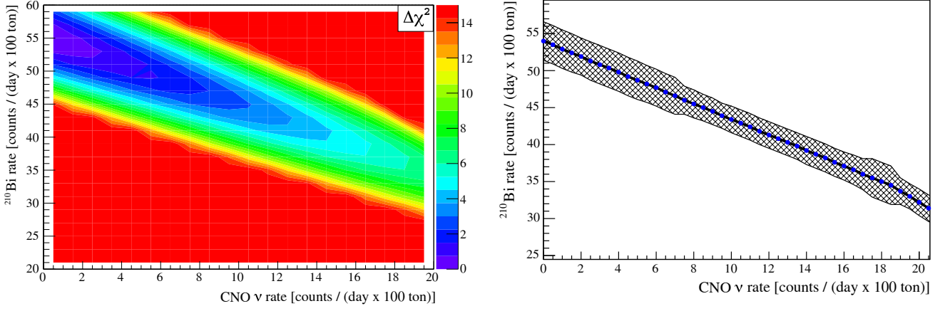
FIG. 74. Correlation between CNO- \nu and ^{210}\text{Bi} rates. Left: \Delta\chi^2 map obtained from a likelihood-ratio test between the likelihood of the best-fit result and the maximum likelihood returned by the fit when the ^{210}\text{Bi} and CNO- \nu interaction rates are fixed to different values. The right column gives the colors corresponding to \Delta\chi^2 values; note that the same red color has been used to plot all \Delta\chi^2 \geq 14 values to allow to visualize color variations in the relevant region of the plot. The plot has been obtained using N_h energy estimator. The pep - \nu rate is fixed to the standard solar model prediction. Right: ^{210}\text{Bi} interaction rate returned by the fit for different (fixed) CNO- \nu interaction rates. The shaded area is the statistical uncertainty.
