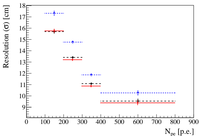
FIG. 12. Resolution ( \sigma ) of the reconstructed x (solid red), y (dashed black), and z (dotted blue) coordinates as a function of energy (in number of photoelectrons) for events from calibration sources placed in the center of the detector.
