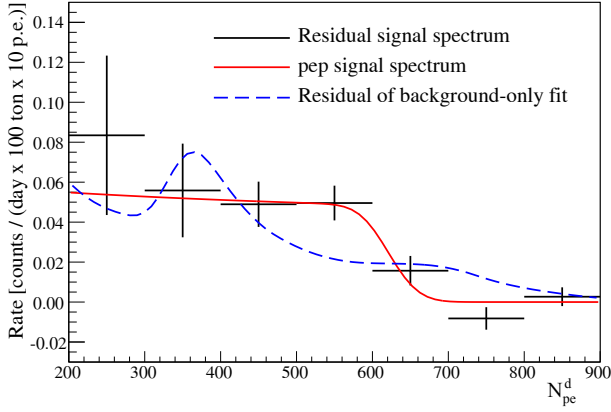
FIG. 76. Residuals after the best-fit values of all species except the signal from pep and CNO solar neutrinos are subtracted from the data energy spectrum (black data points). The e^- recoil spectrum due to pep-\nu is shown in solid-red line. A second fit has been performed excluding the pep and CNO signals. The dashed blue line gives the resulting best-fit spectrum, after the subtraction of the best estimates for the backgrounds, as obtained from the fit used for the signal extraction. The two isotopes showing a significant difference in the output of the background only fit and in the one with the solar neutrinos are ^{210}\text{Bi} and ^{234m}\text{Pa} .
