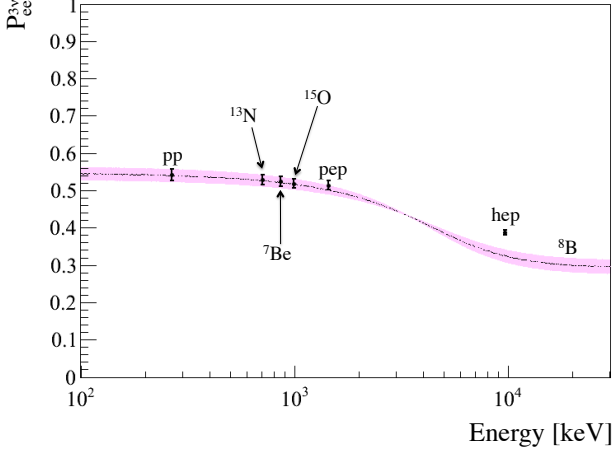
FIG. 83. Electron neutrino survival probability as a function of neutrino energy according to MSW–LMA model, see Eq. 94. The pink band is for ^8\text{B} solar neutrinos, considering their production region in the Sun. The other points represent other solar neutrino fluxes, considering their proper production regions, and reported for mono-energetic ^7\text{Be} (862 keV) and pep (1444 keV) neutrinos and for the mean energies of fluxes with continuous energy spectrum: pp (267 keV), ^{13}\text{N} (707 keV), ^{15}\text{O} (997 keV), and hep (9625 keV).
