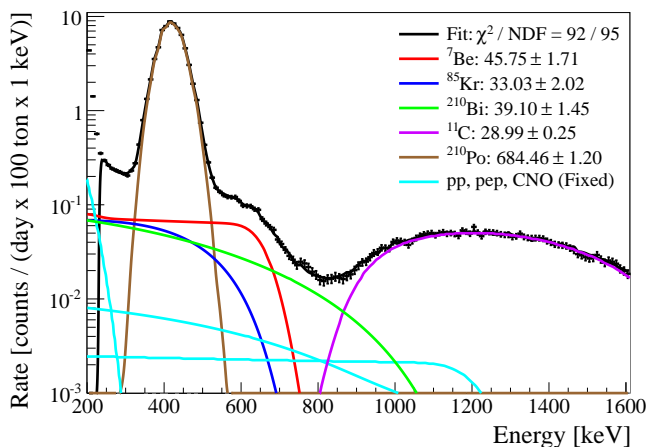
FIG. 54. Example of fit of the energy spectrum obtained using the analytical method without \alpha - \beta statistical subtraction. The fit was done using the N_p energy estimator. After the fit, the horizontal axis was converted into energy scale in keV. The values of the best-fit parameters, the rates of individual species, are given in cpd/100 ton.
