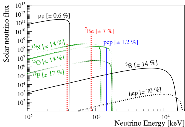
FIG. 1. Energy spectrum of solar neutrinos. The spectral shapes are taken from [1] while the flux normalisation from [2]. The vertical axis report the flux in \text{cm}^{-2} \text{s}^{-1} (10^3 \text{ keV})^{-1} for the continuous neutrino spectra, while in \text{cm}^{-2} \text{s}^{-1} for the mono-chromatic lines ( {}^7\text{Be}-\nu at 384 and 862 keV, shown as red dotted lines, and pep-\nu at 1440 keV, shown as a blue continuous line). The numbers in parenthesis represent the theoretical uncertainties on the expected fluxes.
