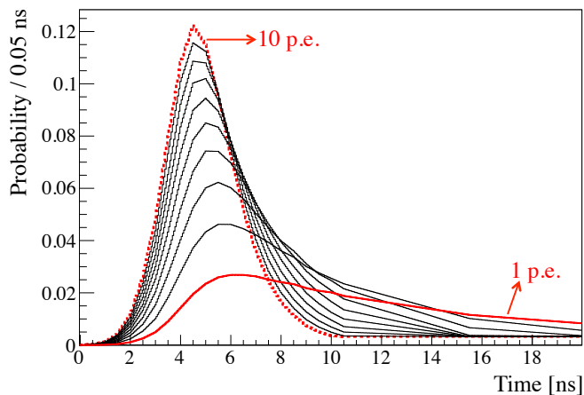
FIG. 11. Probability density functions for detected hits as a function of time elapsed from the emission of scintillation light. Different curves are for increasing values of the hit charge q_i^j collected at the phototube: from 1 p.e. (red solid curve) to 10 p.e. (red dashed curve).
