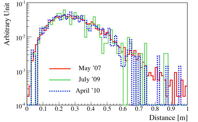
FIG. 62. Absolute distance between {}^{214}\text{Bi} - {}^{214}\text{Po} fast coincidence events in three periods: May 2007 (solid red), July 2009 (solid green), and April 2010 (dotted blue).
