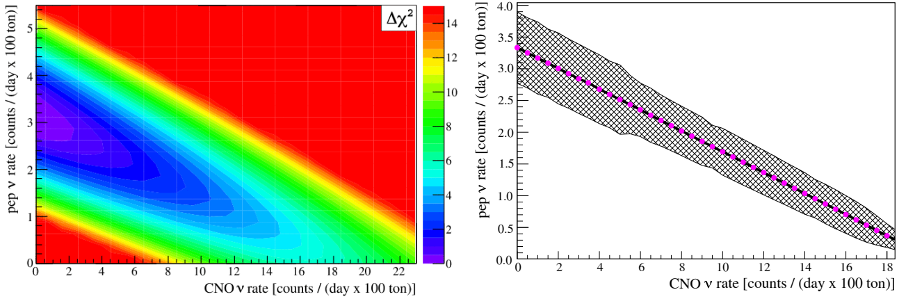
FIG. 75. Correlation between the pep and CNO neutrino rates. Left: \Delta\chi^2 map obtained from a likelihood-ratio test between the likelihood of the best-fit result and the maximum likelihood returned by the fit when pep and CNO neutrino interaction rates are fixed to different values. The right column gives the colors corresponding to \Delta\chi^2 values; note that the same red color has been used to plot all \Delta\chi^2 \geq 14 values to allow to visualize color variations in the relevant region of the plot. The numerical values of this map are given in Table XXIII. The plot has been obtained using N_{pe}^d energy estimator; we get similar and consistent numbers using the N_h variable. Right: pep - \nu interaction rate returned by the fit for different (fixed) CNO neutrino interaction rates. The shaded area is the statistical uncertainty.
