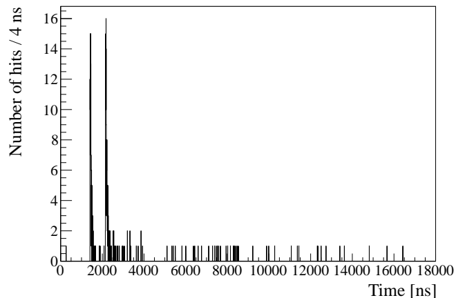
FIG. 7. An example of a single data acquisition gate (so called event) containing two well separated clusters, which are due to two different interactions inside the scintillator.
