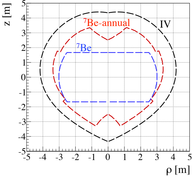
FIG. 17. \rho - z projection of the IV as of May 3 rd , 2009 (black). The blue curve shows the shape of the 75 ton FV used for the measurement of the {}^7\text{Be}-\nu interaction rate. The red curve illustrates the profile of the FV used for the {}^7\text{Be}-\nu annual modulation analysis.
