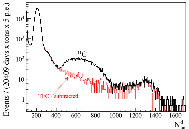
FIG. 40. Energy spectra ( N_{pe}^d energy estimator) before (black) and after (red) the application of the TFC technique for ^{11}\text{C} removal. Both spectra are normalized to the same exposure.
