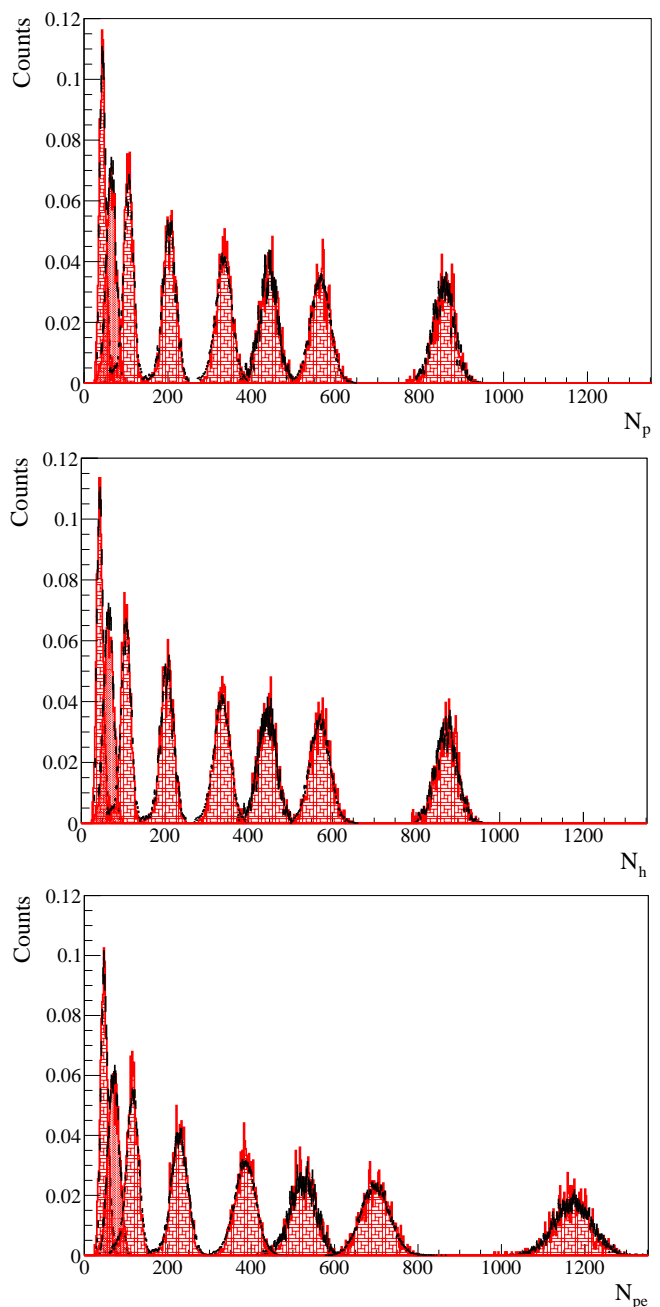
FIG. 47. Energy spectra ( N_p , N_h , and N_{pe}^d variables) of the calibration sources placed in the detector's center: measured data (black lines) versus the Monte Carlo simulation (areas dashed with red lines). The peaks represent (from the left to the right) the total \gamma decay energy of ^{57}\text{Co} , ^{139}\text{Ce} , ^{203}\text{Hg} , ^{85}\text{Sr} , ^{54}\text{Mn} , ^{65}\text{Zn} , ^{40}\text{K} , and ^{60}\text{Co} .
