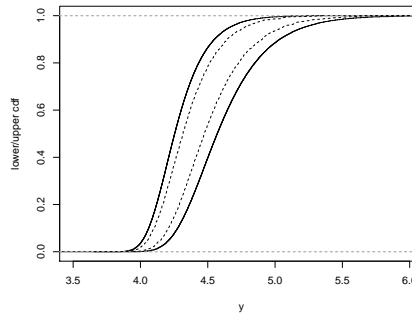
Fig. 5 Lower and upper cdfs of the type-II PBF for the sea-level example (solid lines). The type-I lower and upper cdf are shown as broken lines.
