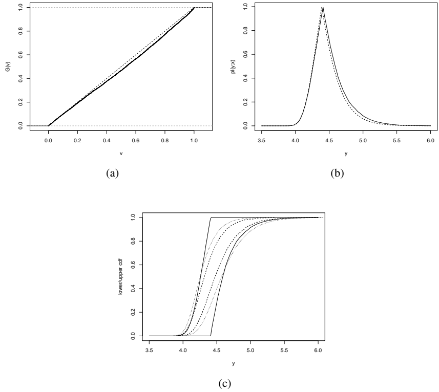
Fig. 7 Sea-level example. (a): Bootstrap estimate of the cdf G of \tilde{V} = F(Y, \hat{\theta}(X)) ; (b): Contour function of the type-III PBF (solid line), and contour function induced by the plug-in distribution (interrupted line); (c): Lower and upper cdfs of the type-III PBF (solid lines). The type-I and type-II lower and upper cdf are shown, respectively, as interrupted and dotted lines.
