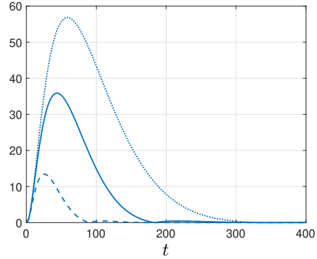
Fig. 7. Evolution of \|(\varepsilon, \eta)\|_Z for the initial condition in (25) obtained for different designs: (\vartheta, \mu) = (1, 1.3) (dashed line), (\vartheta, \mu) = (0.5, 2.2) (solid line), and (\vartheta, \mu) = (1, 2.2) (dotted line).
