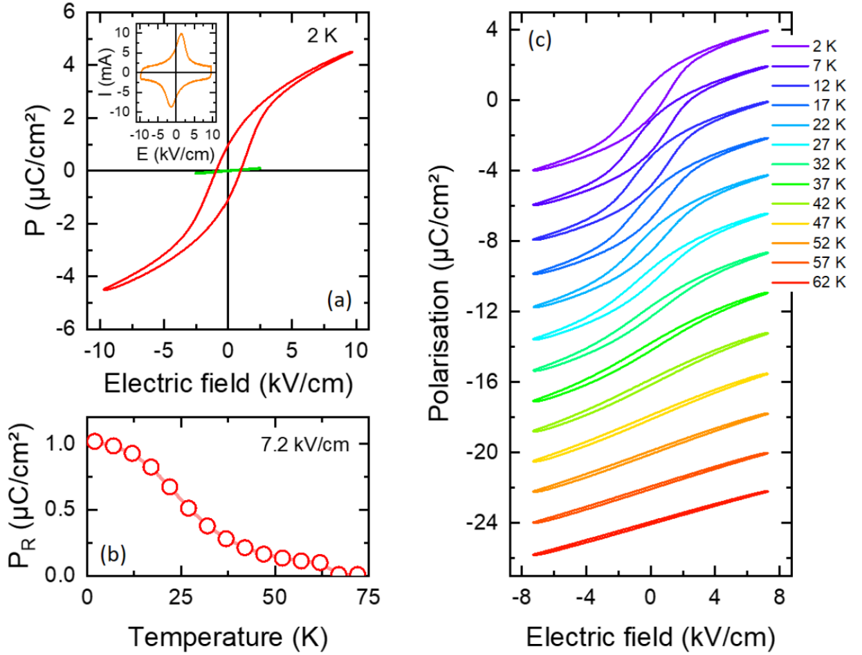
Fig. 3. Electric polarisation measurements. (a) Polarisation vs voltage curves measured on a \text{Al}(1.8 \text{ nm})//\text{STO} sample. The green curve corresponds to the polarisation loop measured with a maximum field of 2 kV/cm. Inset: Corresponding current vs voltage curve. (b) Temperature dependence of the remanent polarisation P_R . (c) Polarisation loops at different temperatures.
