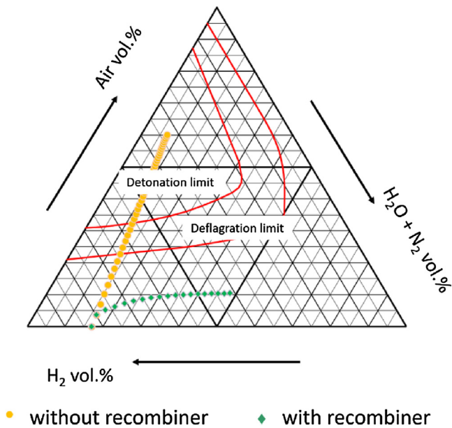
Fig. 9. Course of accident with and without recombinder.
