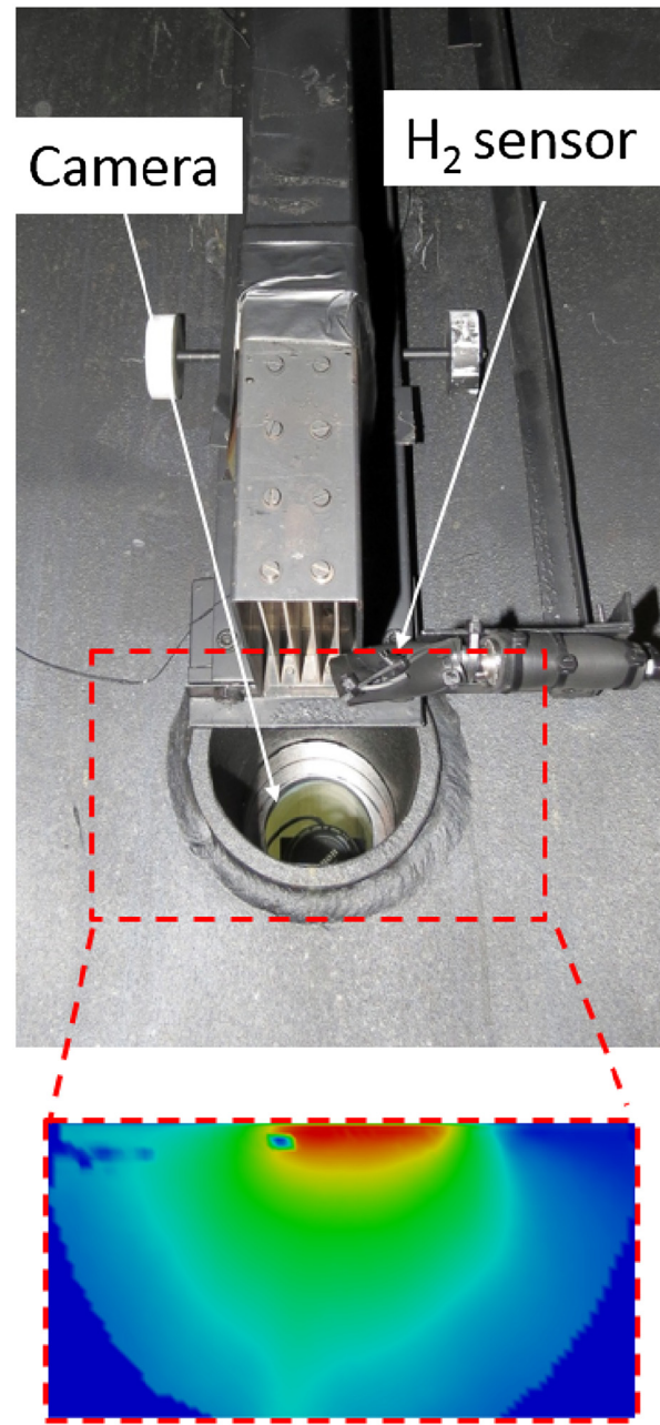
Fig. 4. \text{H}_2 sensor and PIV measurement at the PAR inlet.
