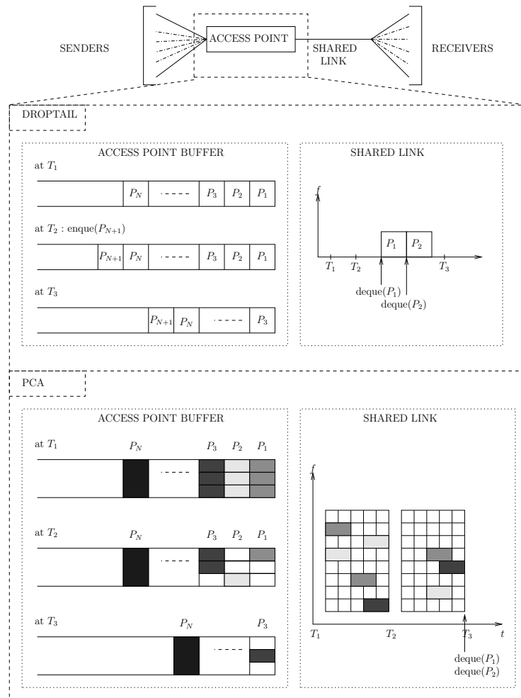
Fig. 2. Capacity allocation: enque() and deque()
