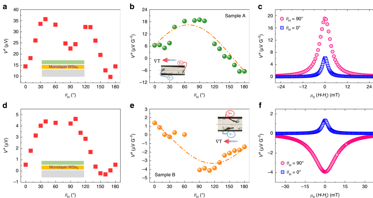
Fig. 4 VNE in the monolayers WSe 2 . Sample A: a V 1 s (Seebeck effect) and b V a = V 1 a + V t a (ISHE and Nernst-related effects) voltages as a function of the angle θ H ; c Parallel (V a = V 1 a , θ H = 0°, ISHE) and perpendicular (V a = V t a , θ H = 90°, Nernst-related effects) configurations. Sample B: d V 1 s and e V a = V 1 a + V t a as a function of the angle θ H ; f Parallel (V a = V 1 a , θ H = 0°, ISHE) and perpendicular (V a = V t a , θ H = 90°, Nernst-related effects) configurations. The insets in b and e are optical images showing longitudinal distances of 1.3 and 0.3 mm between the contacts of the samples A and B, respectively and the dash-dotted lines are guide for the eye. The insets of a and d show the schematics of the stacks (color code: gray for SiC-graphene substrate, orange for WSe 2 and green for Al/NiFe/Al).
