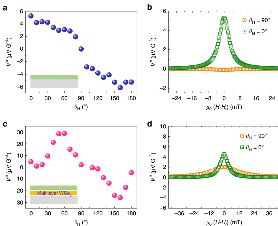
Fig. 5 VNE in the reference (sample C) and in the multilayer WSe 2 (sample D). Sample C: a V a = V 1 a + V t a as a function of the angle θ H ; b Parallel (V a = V 1 a , θ H = 0°, ISHE) and perpendicular (V a = V t a , θ H = 90°, Nernst-related effects) configurations. Sample D: c V a = V 1 a + V t a as a function of the angle θ H ; d Parallel (V a = V 1 a , θ H = 0°, ISHE) and perpendicular (V a = V t a , θ H = 90°, Nernst-related effects) configurations. The insets of a and c show the schematics of the stacks (color code: gray for SiC-graphene substrate, orange for WSe 2 and green for Al/NiFe/Al).
