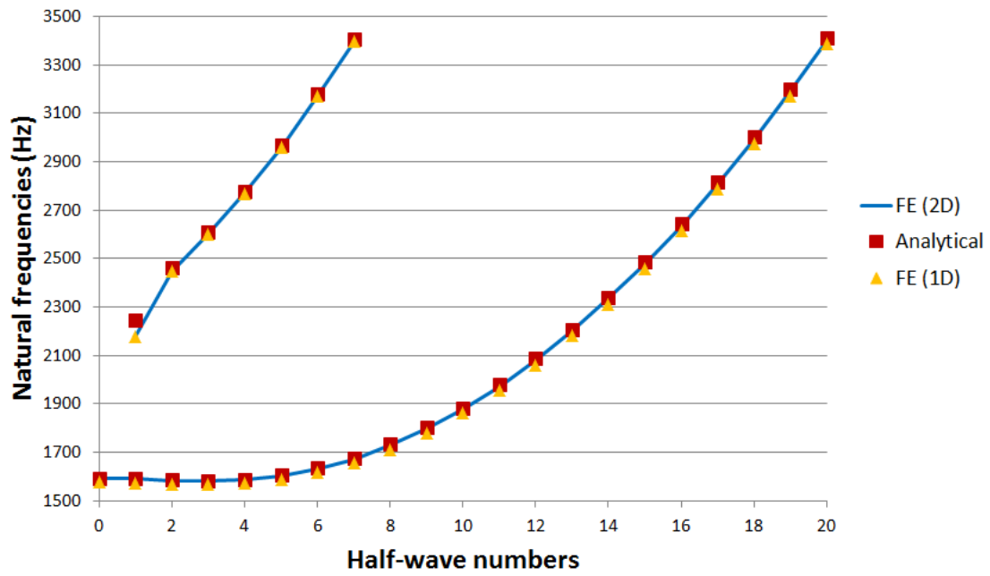
(b) Symmetric modes
