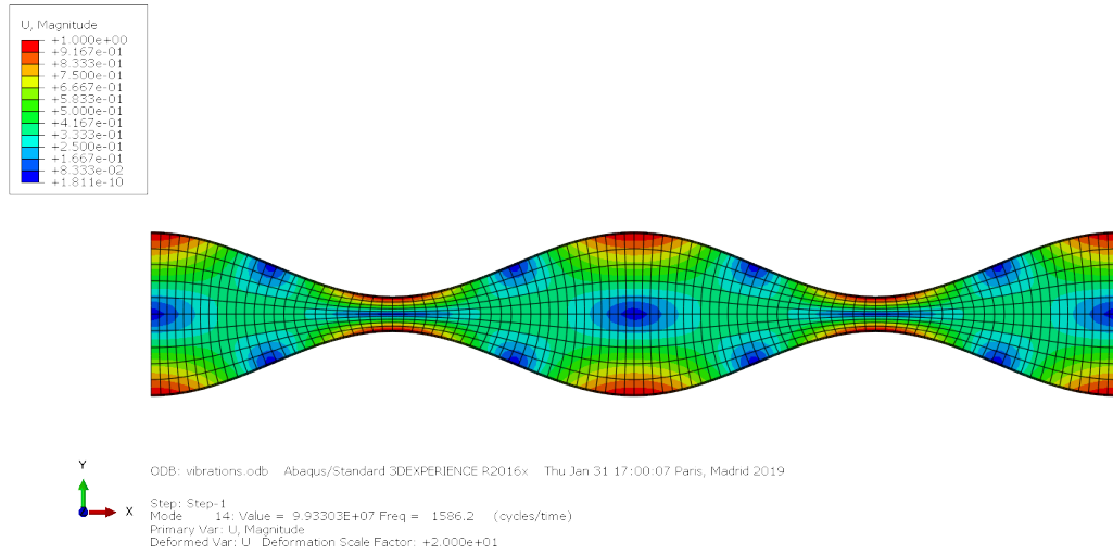
(a) First symmetric mode ( f = 1586 \text{ Hz} )
