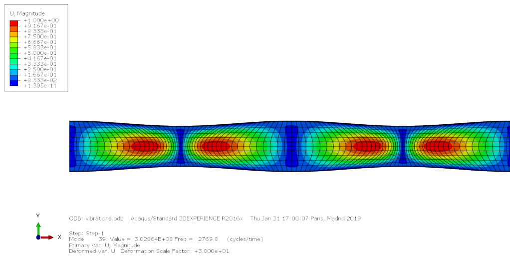
(b) Second symmetric mode ( f = 2770 \text{ Hz} )
