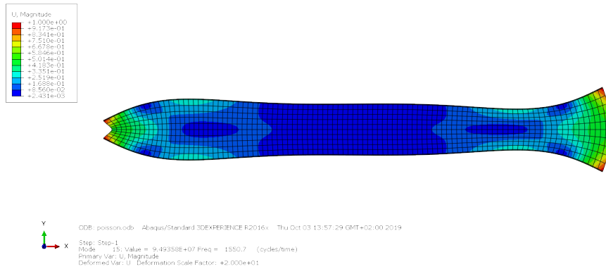
(b) Mode 12 with 2D model ( f = 1551 \text{ Hz} )
