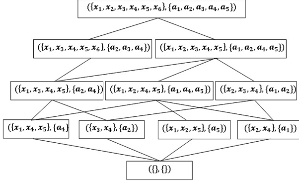
Figure 1. Lattice \mathcal{L}_{N\Pi} for K_S .
