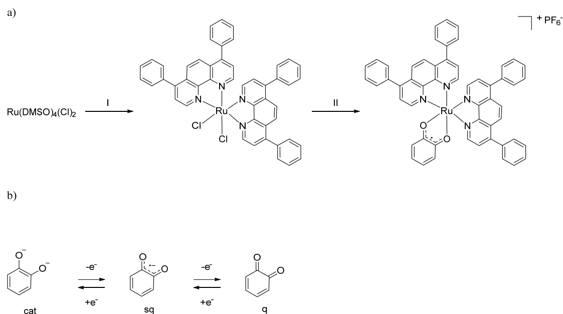
Scheme 1. a) Synthesis of [Ru(DIP) 2 (sq)](PF 6 ) . I) DIP, LiCl, DMF, reflux, 24 h, 78%; II) (i) NaOH, catechol 2-propanol, reflux, 24h; (ii) air, 2 h; (iii) NH 4 PF 6 , 2-propanol/H 2 O (1:8), 19%. b) Catecholate (cat) and its oxidised forms, semiquinonate (sq) and quinone (q).
