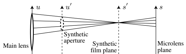
Figure 5: Conceptual model for synthetic photography, shown in 2D. The u and s planes are the physical surfaces in the light field camera. u' is a virtual plane containing the synthetic aperture shown in dotted line, and s' is the synthetic film plane, together forming a synthetic camera. Note that these planes need not be between the acquisition planes. The image value that forms on the convergence point on the synthetic film is given by the sum of the illustrated cone of rays (see Equation 5). We find these rays in the acquired light field by their intersection points with the u and s planes.
