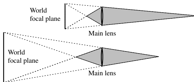
Figure 6: The space of locations (shaded regions) for a synthetic pinhole camera that result in a synthetic photograph without vignetting. The same optical system is depicted at two focus settings (resulting in different image magnifications, higher on top). Note that the space shrinks relative to the distance to the scene as the magnification decreases. Thus, close-up photography (macro photography) results in the greatest ability to move the observer.
