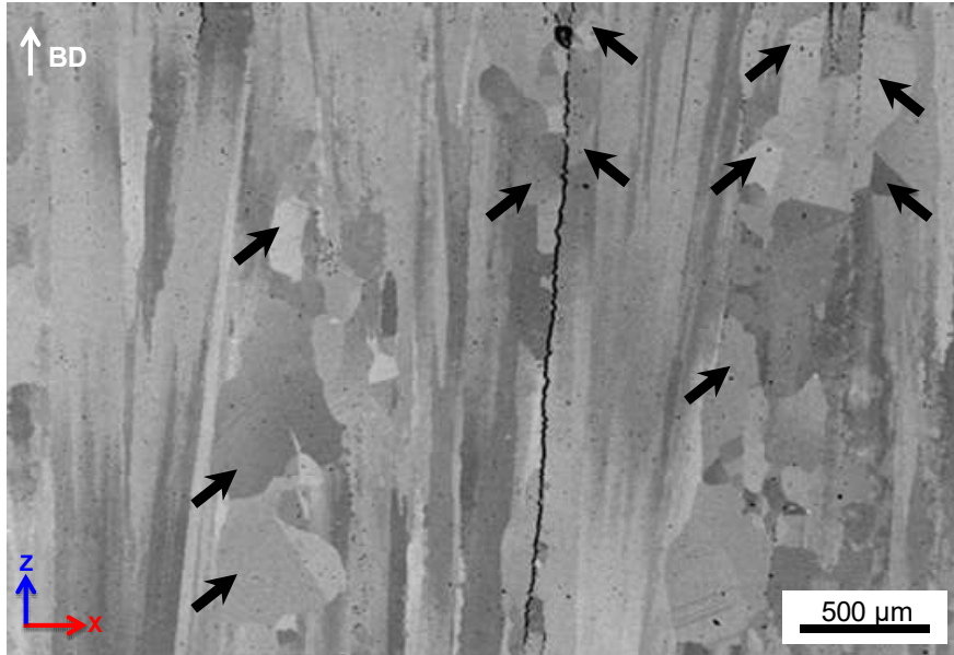
Figure 11. Typical BSE-SEM micrographs after a solutionizing heat treatment: 1190°C/4h followed by air quenching depicting regions where recrystallization occurred (Recrystallized grains are pointed out by black arrows).
